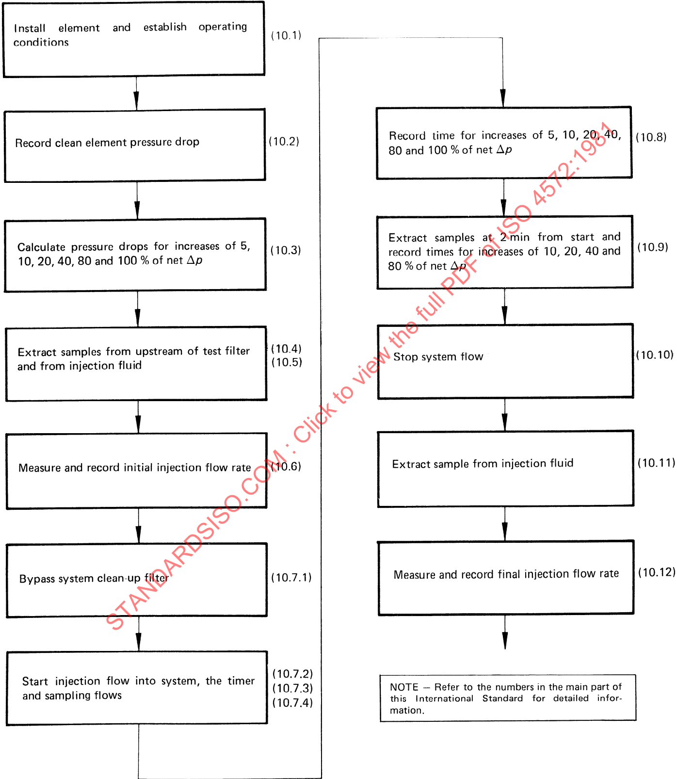
Figure 6 — Procedural diagram for filter performance test
