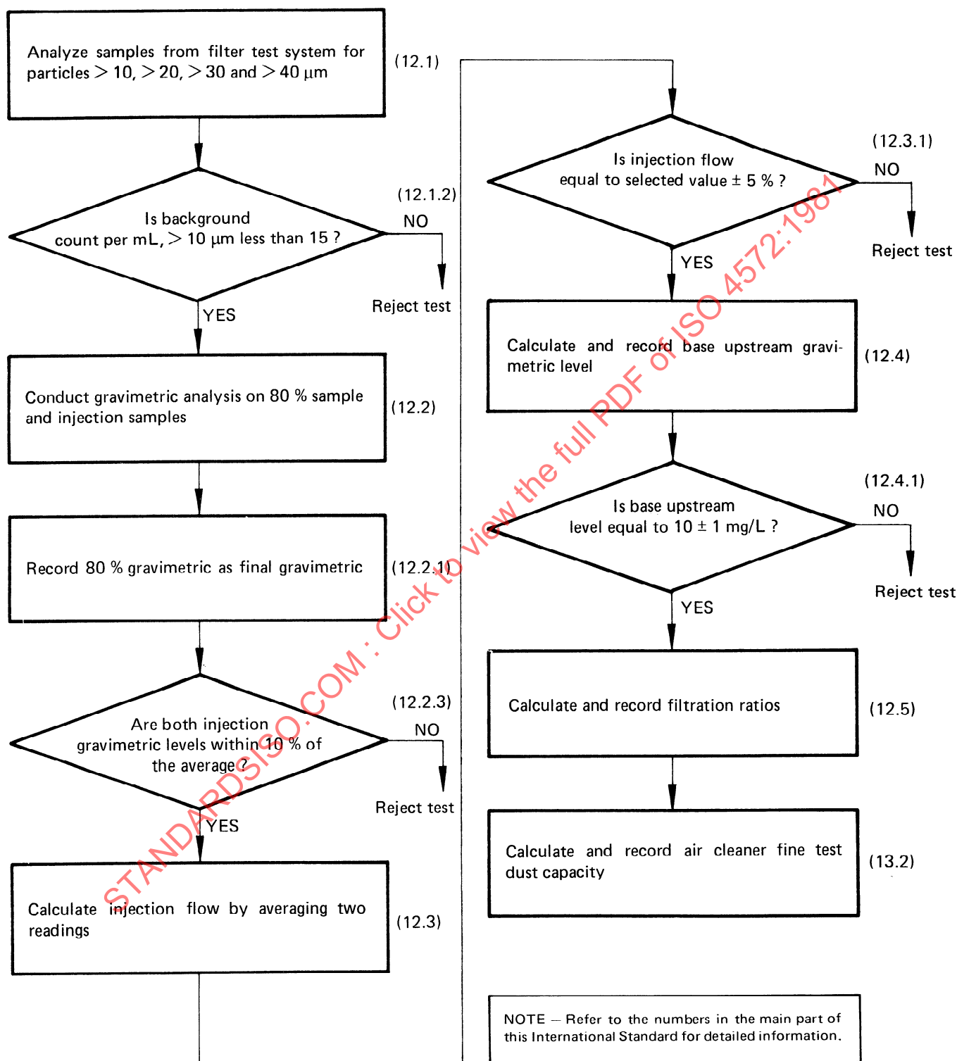
Figure 7 — Procedural diagram for data analysis and presentation
