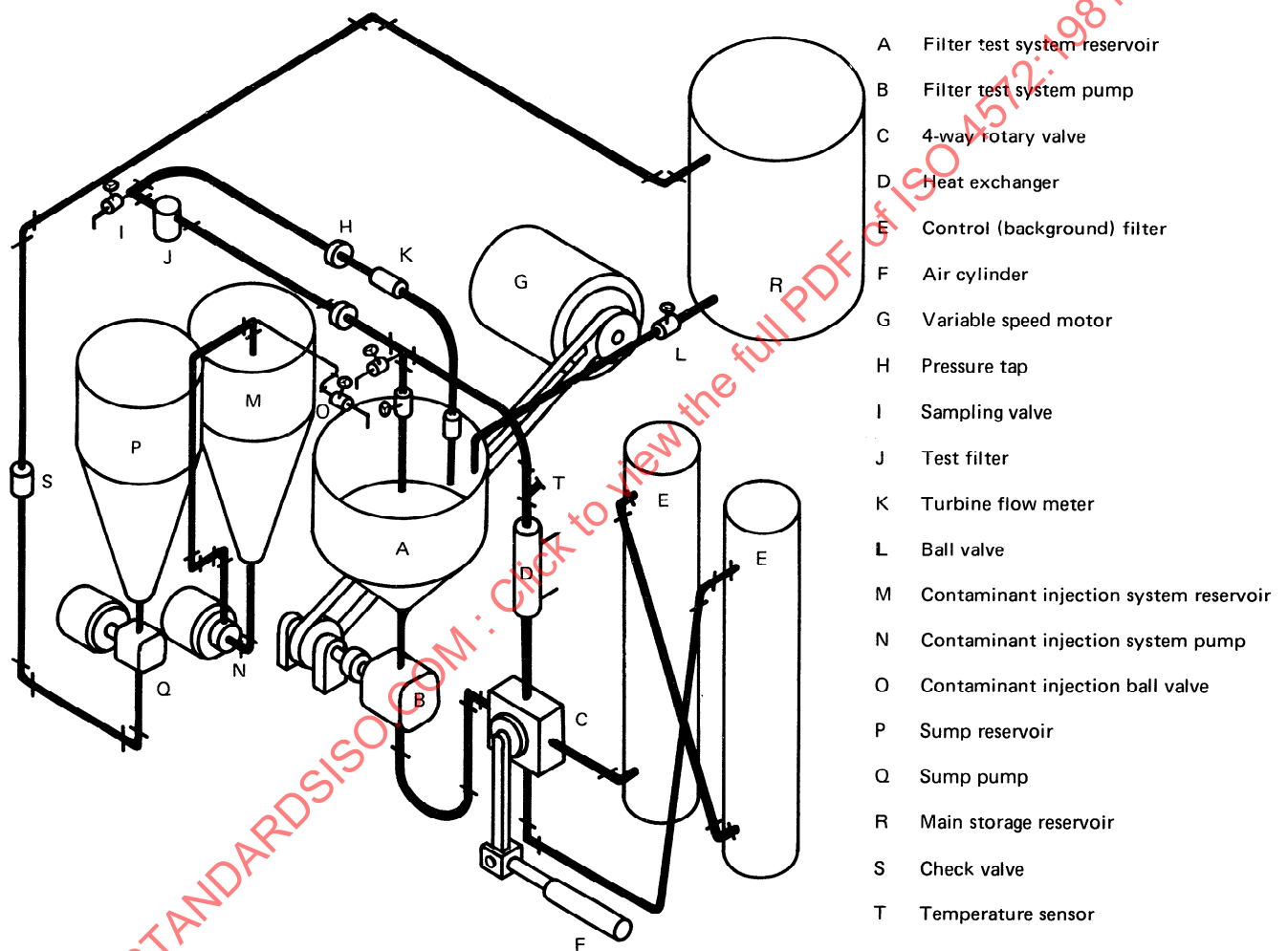
Figure 2 — A typical filter performance test system
