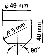
FIGURE 2 — Piston
