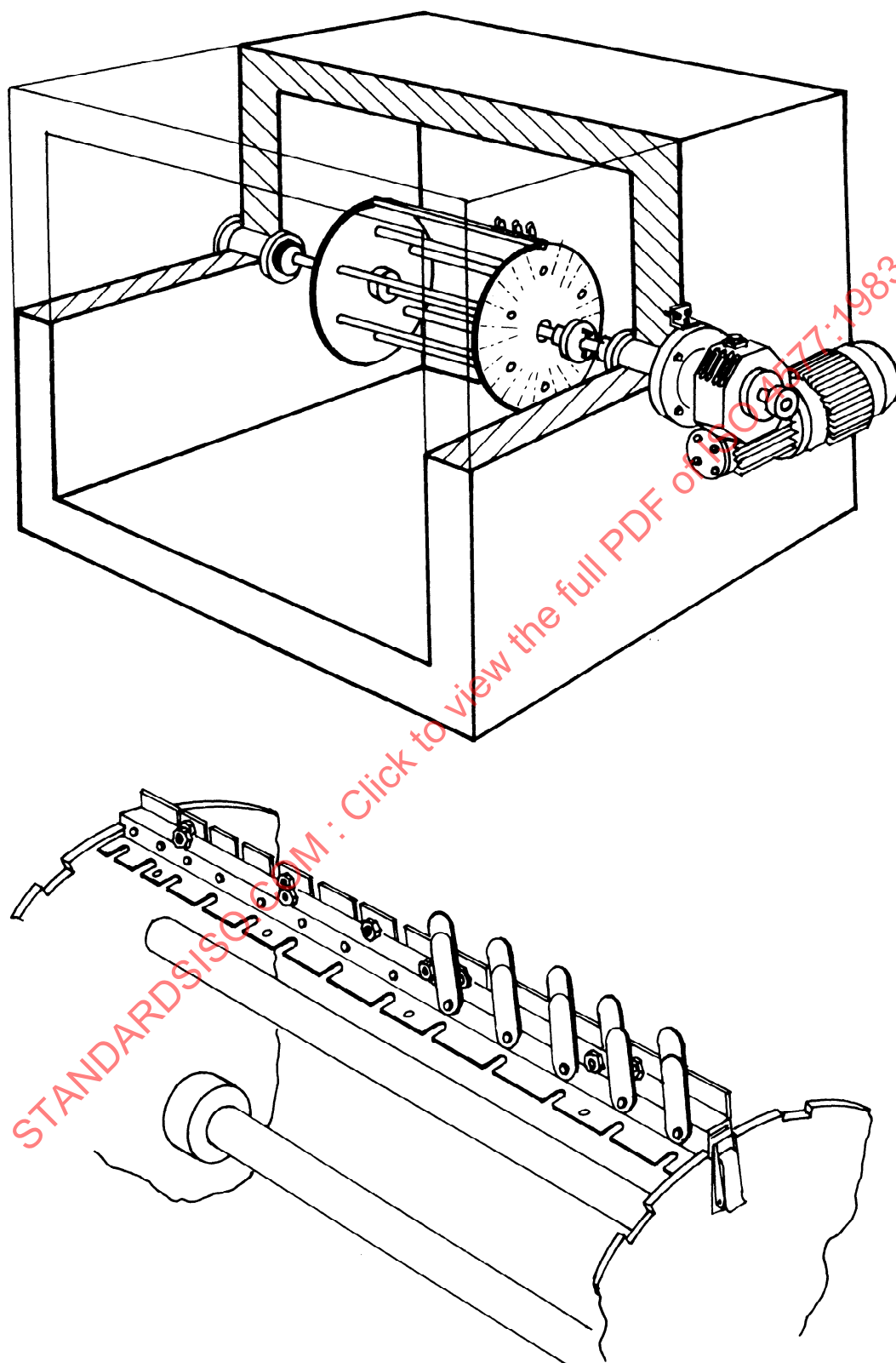
Figure 2 — Uniaxially rotated specimen holder — Drum rotator
