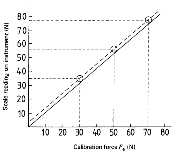
Figure 6 — Example of calibration graph relating actual force to scale value (see 11.5)
