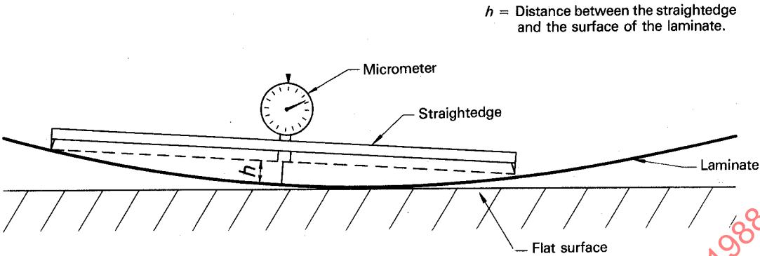
Figure 1 — Example of measuring equipment for warping (see 5.2.1)
