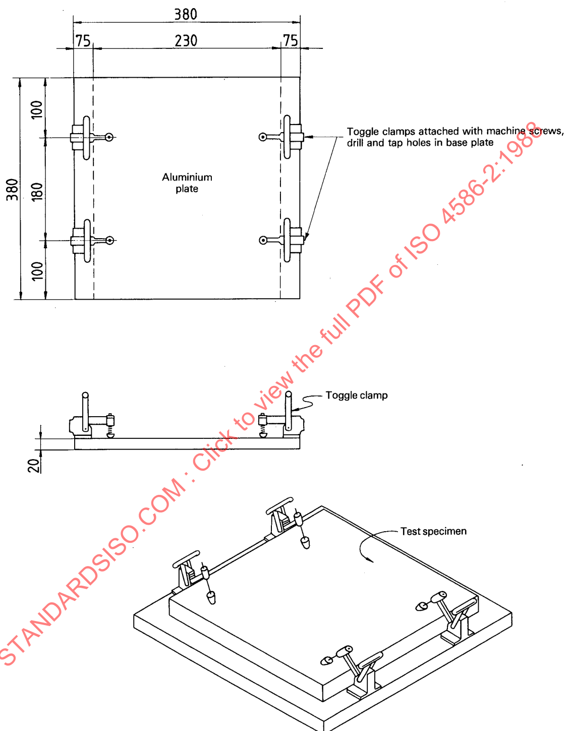
Figure 9 — Clamping frame (see 12.3.3)
