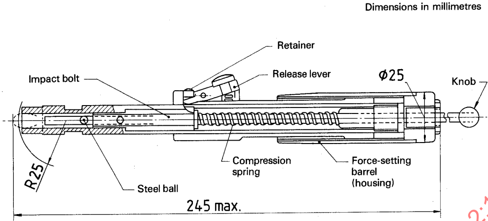
Figure 4 — Impact tester (shown with spring compressed) (see 11.3.1)
