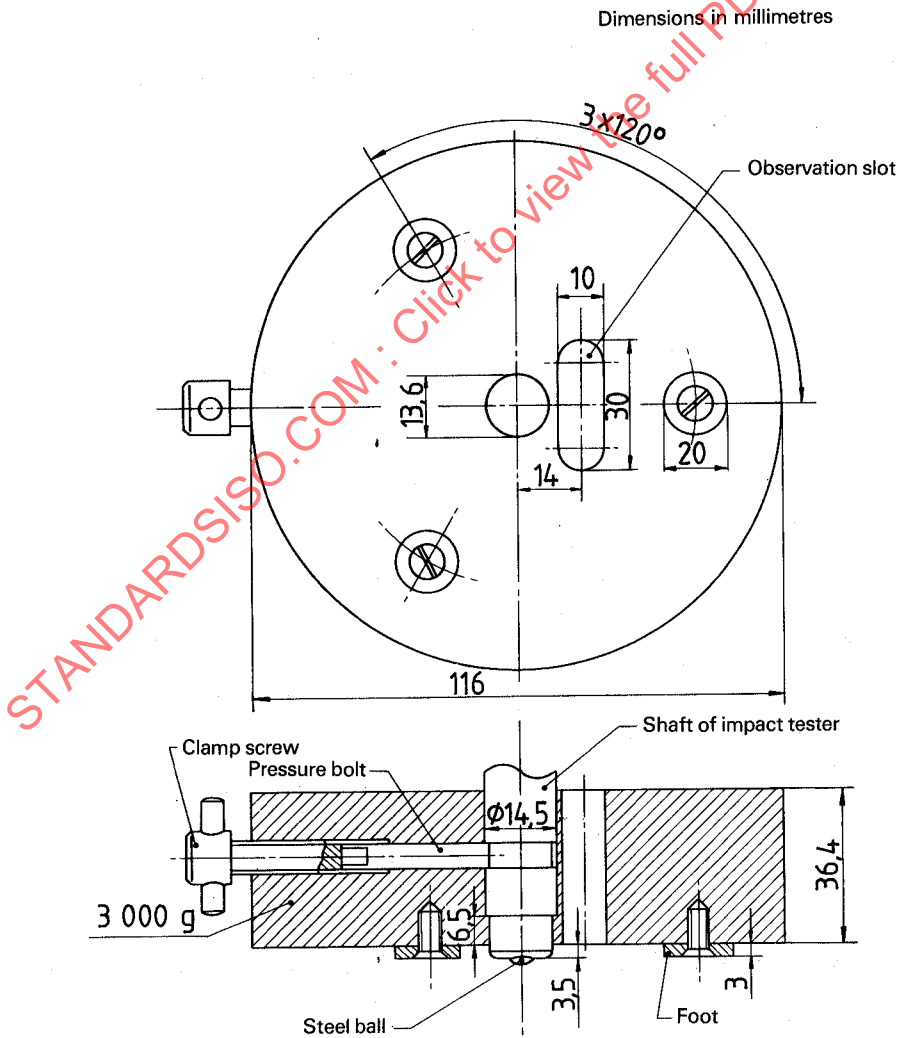
Figure 5 — Support fixture for impact tester (see 11.3.3)
