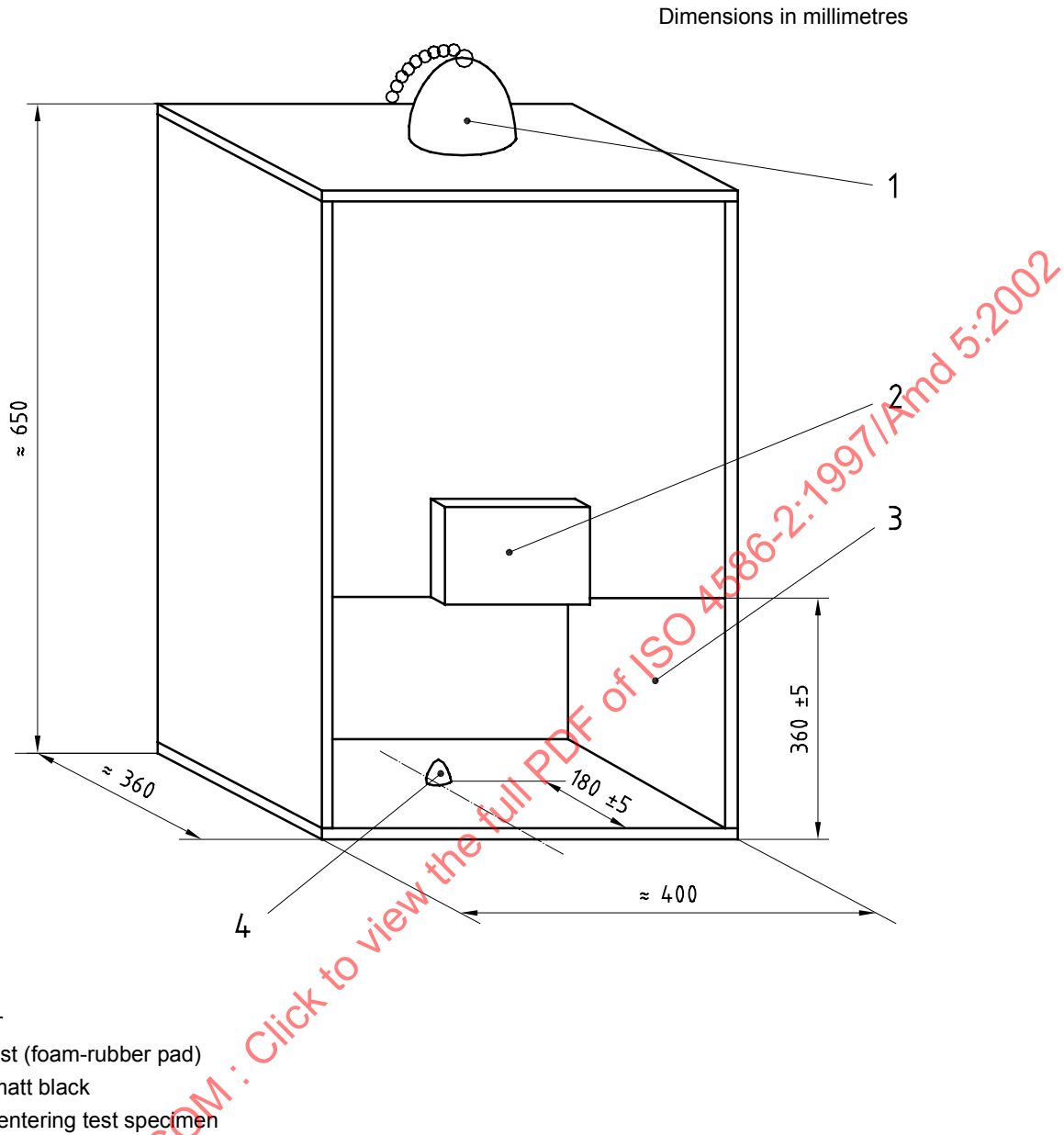
Figure 11 — Example of suitable viewing enclosure (see 14.3.2)
