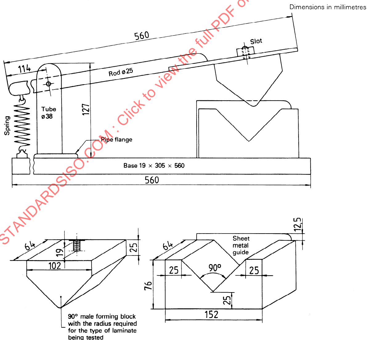
Figure 18 — Forming apparatus (radiant heat test) (Method A) (see 19.2.5)
