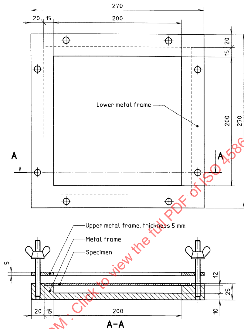
Figure 7 — Clamping frame (see 12.3.3)
