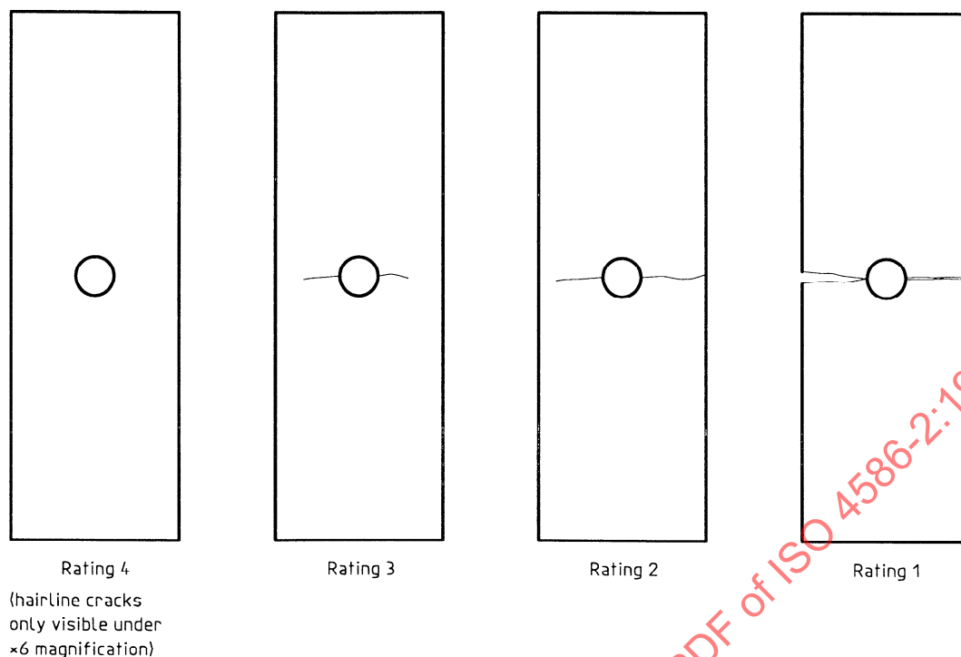
Figure 8c — Classification of types of failure
