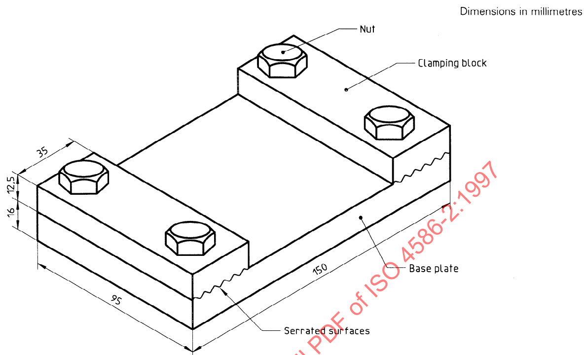
Figure 8 a — Clamping device (mild steel)
