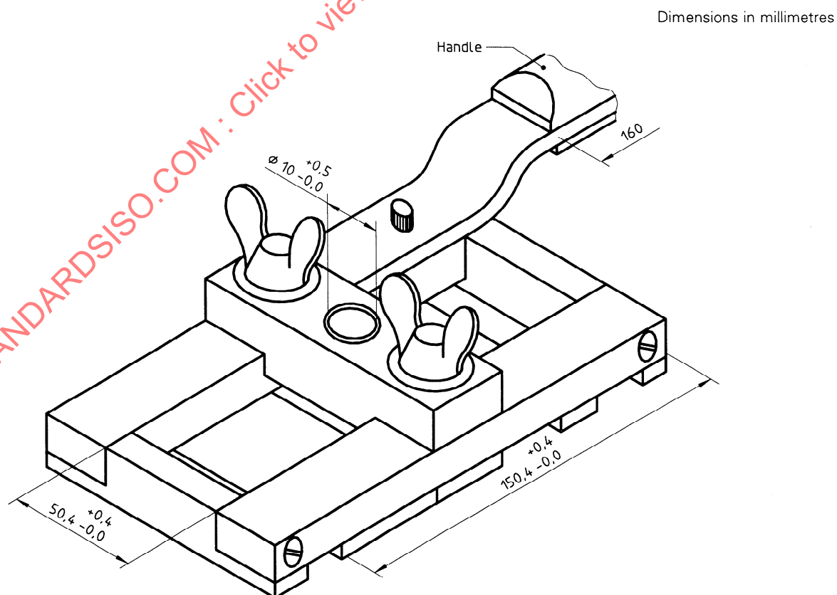
Figure 8 b — Drilling jig (mild steel)
