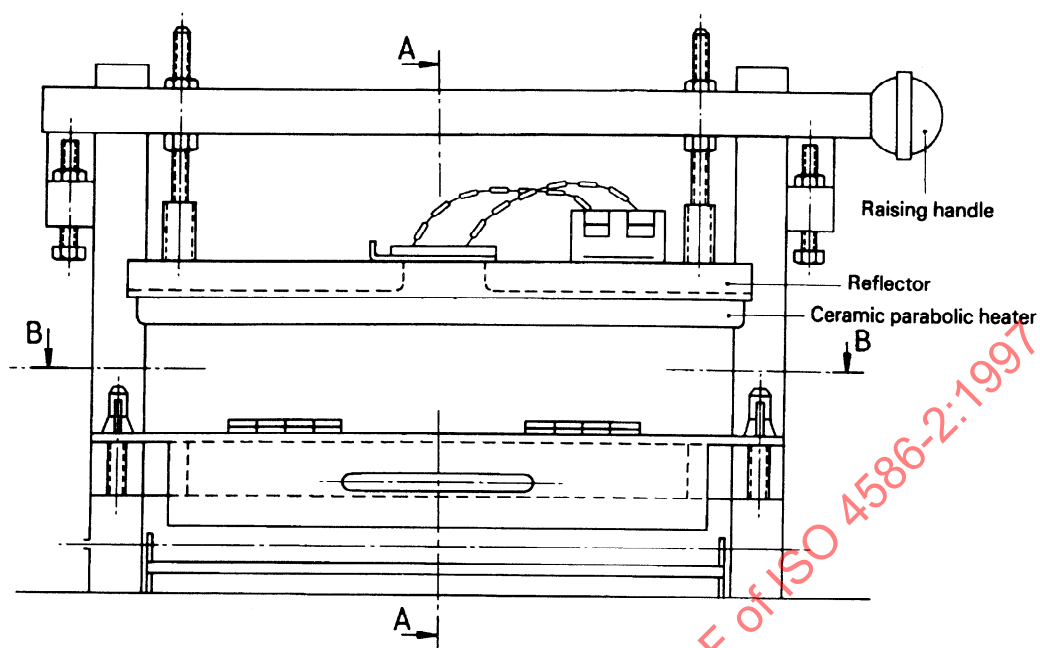
a) Profile
