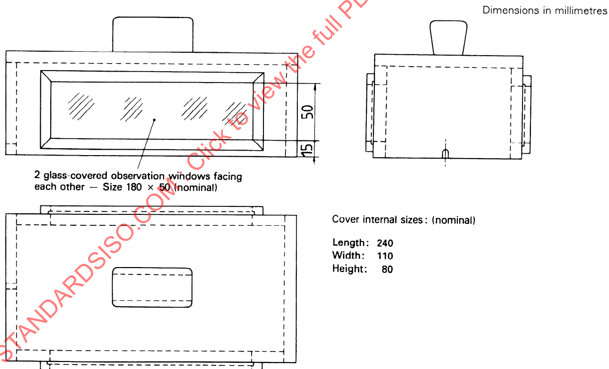
Figure 16 — Apparatus cover (H) for cigarette test (see 18.3.5)
