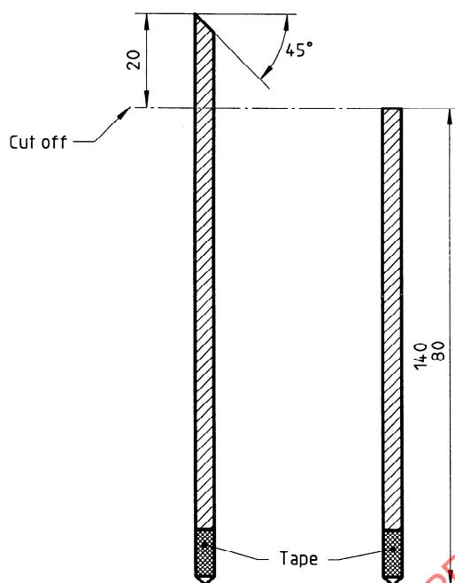
Figure 4 — Rolled specimen
