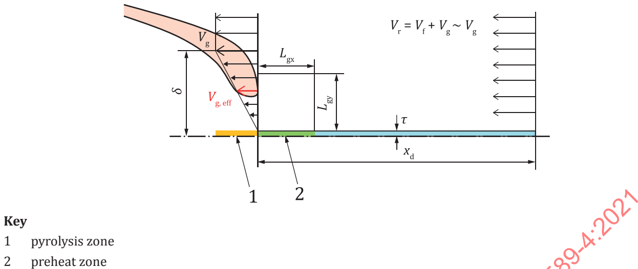
Figure D.2 — Schematic of two-dimensional flame on a solid material
