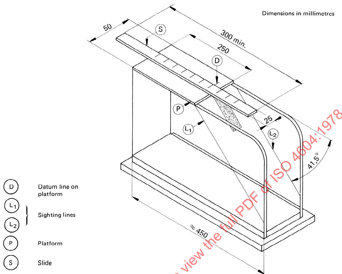
FIGURE 1 — Fixed-angle flexometer for determination of stiffness
