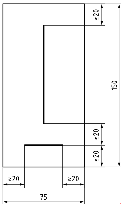
Figure 1 — Arrangement of scribes on test panel
