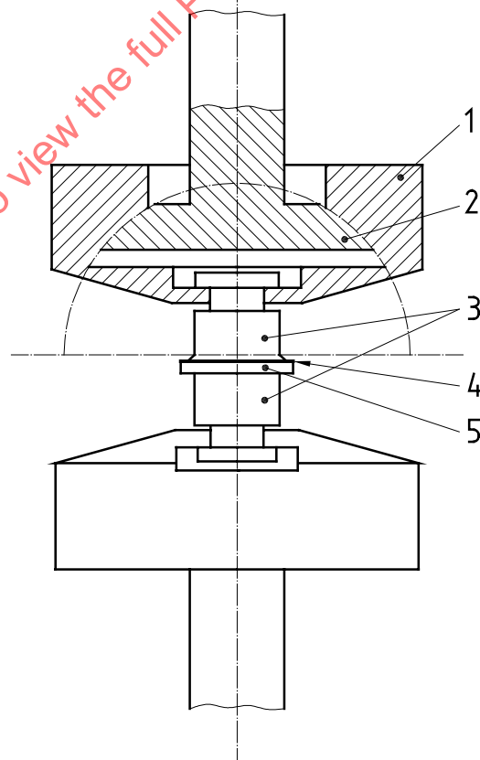
Figure 1 — Example of a suitable test apparatus for the methods described in 9.4.1 and 9.4.3
