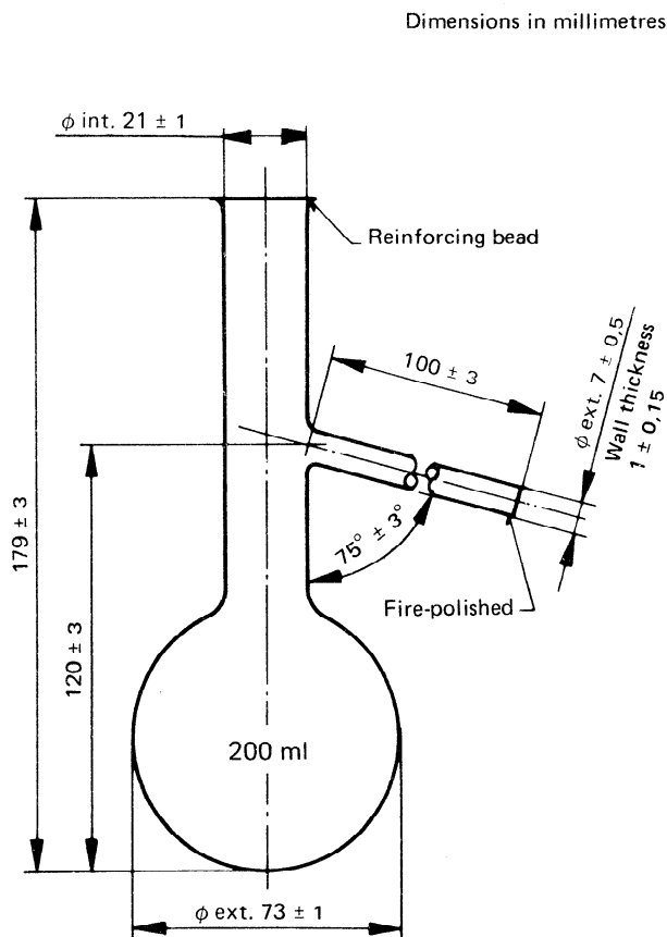
FIGURE 1 — Distillation flask (5.1)
