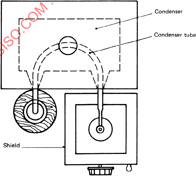
FIGURE 3 — Distillation apparatus using electric heater
