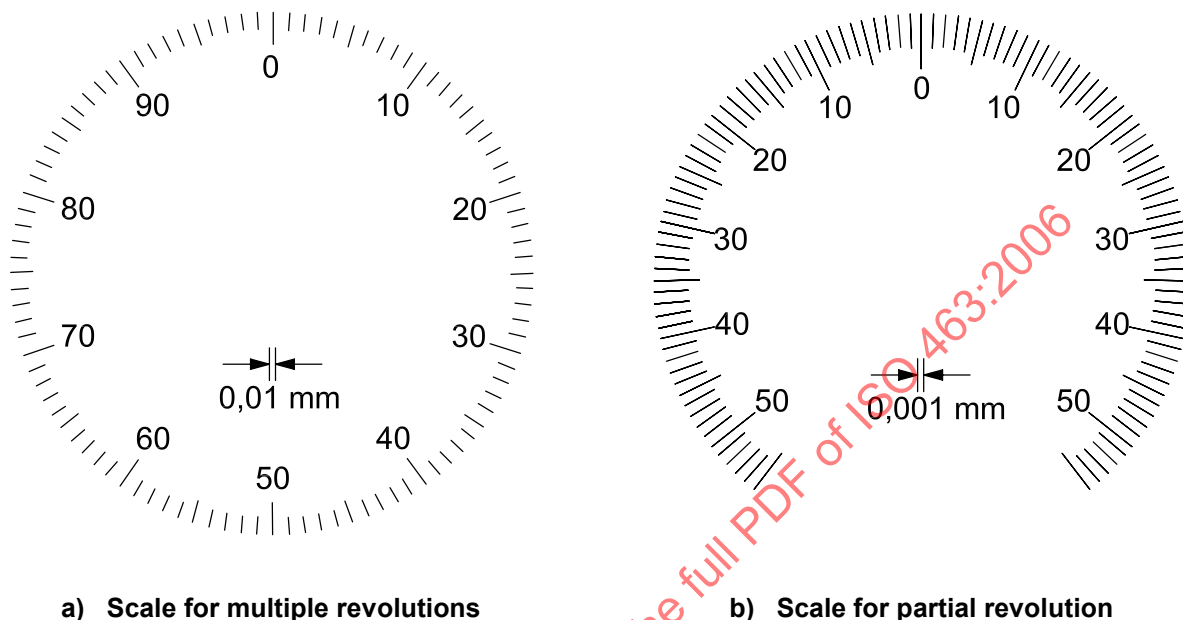
Figure 3 — Examples of scale layouts
