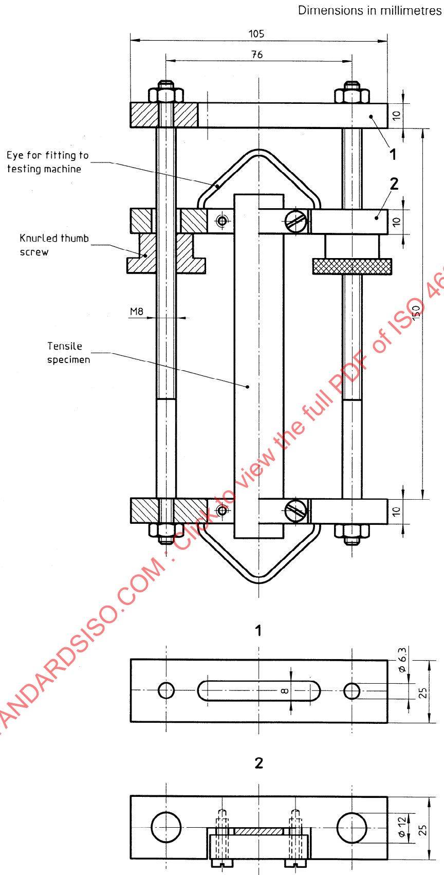
Figure A.1 — Example of an apparatus for determining stress relaxation in tension (the dimensions given are for guidance only)
