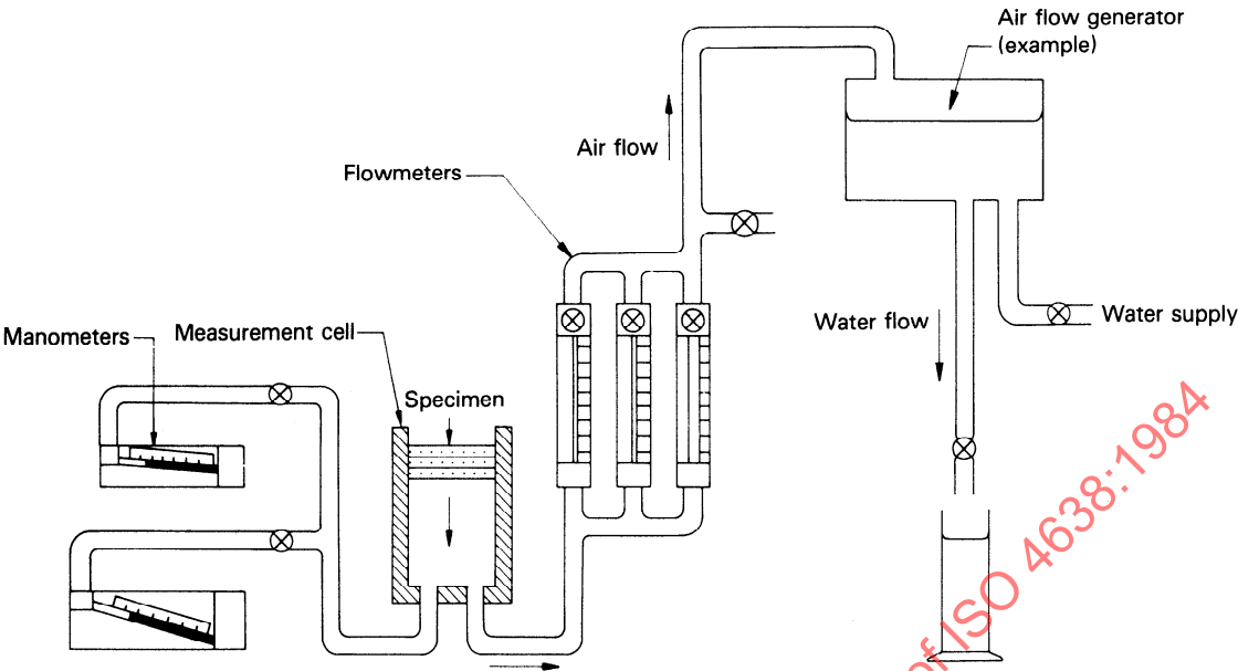
Figure 2 — Schematic diagram of an air flow permeability apparatus
