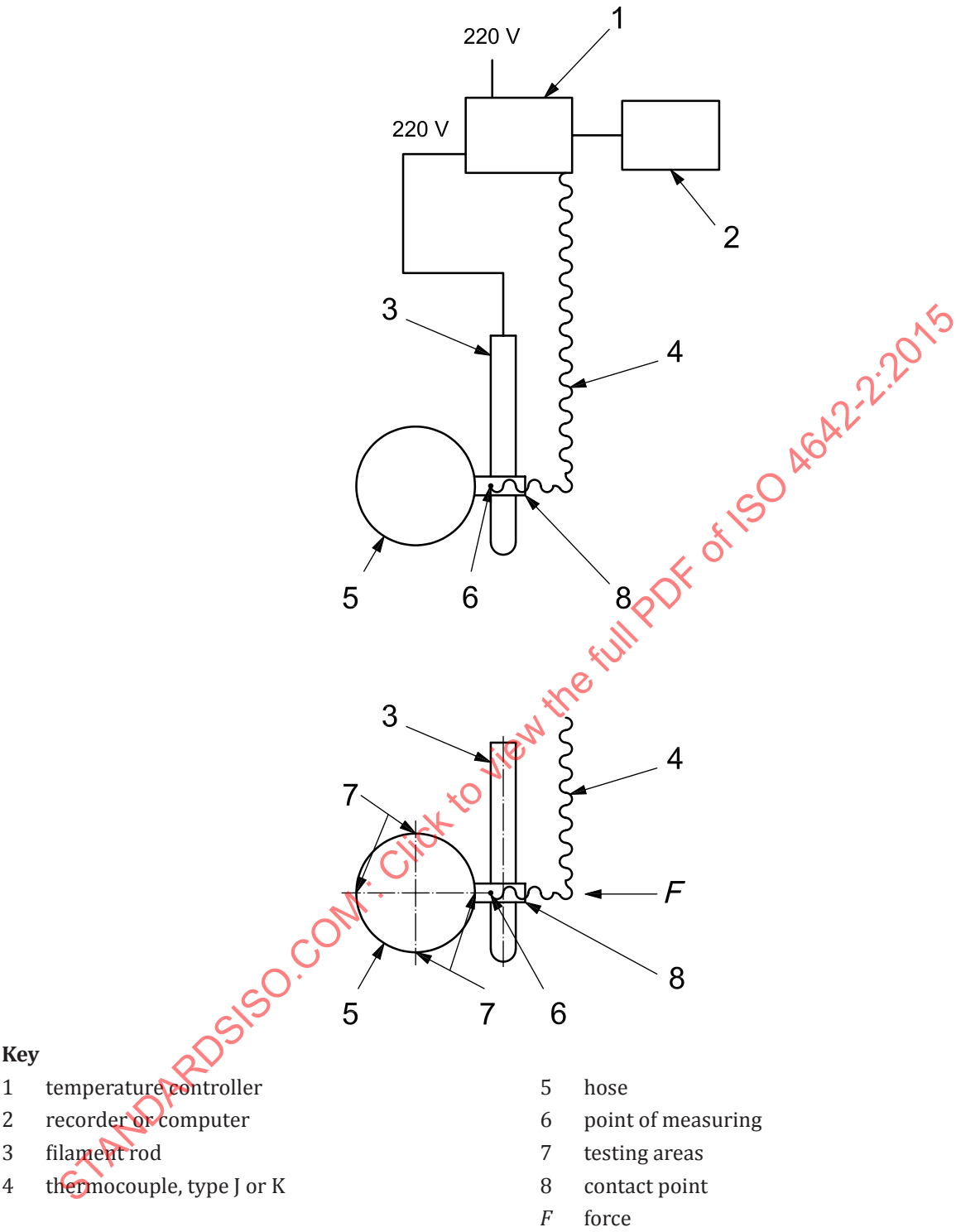
Figure E.2 — Point of contact of filament rod with hose (seen from above)
