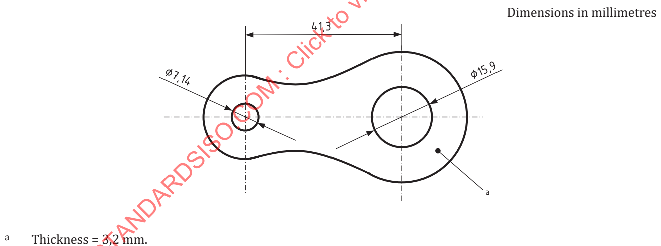
Figure A.1 — Ball support
