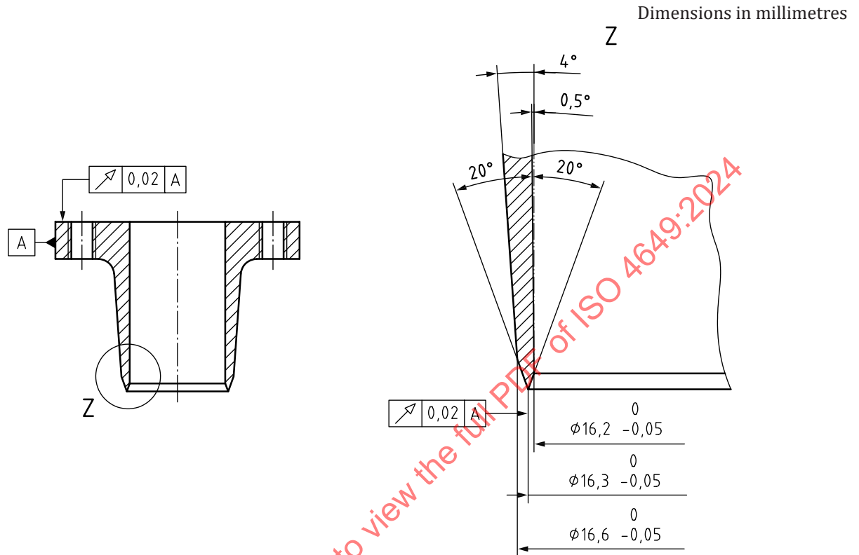
Figure 2 — Example of a hollow drill for test piece preparation
