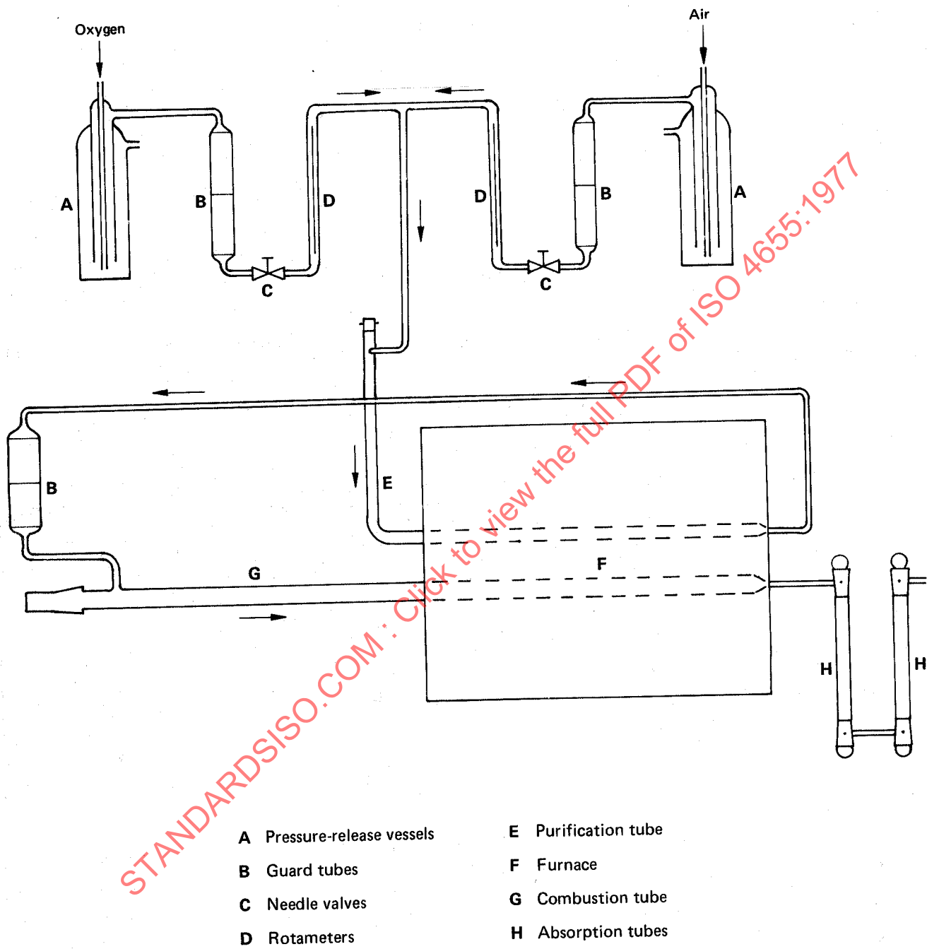
FIGURE 1 — Arrangement of combustion apparatus for carbon/hydrogen method
