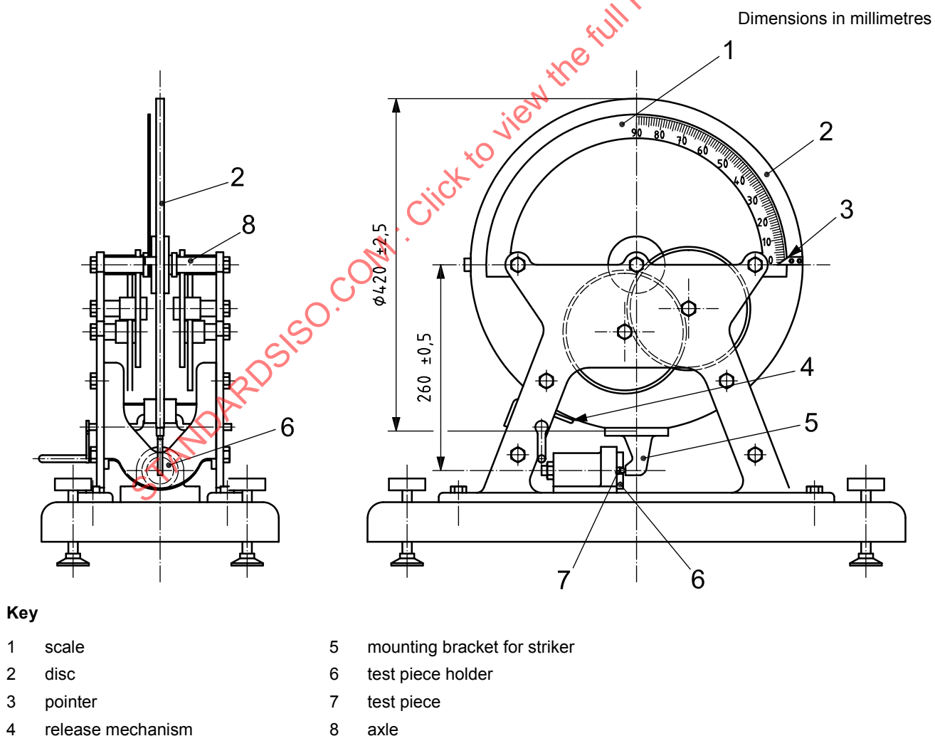
Figure C.1 — Example of a conventional mounting system for a tripsometer
