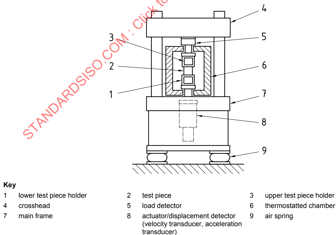
Figure 5 — Example of large-sized test apparatus
