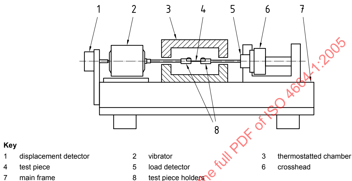
Figure 4 — Example of small-sized test apparatus
