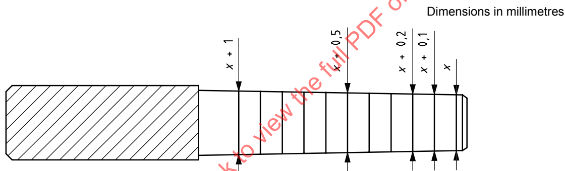
Figure 2 — Tapered gauges
