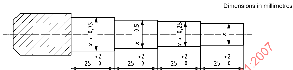
Figure 1 — Plug gauges
