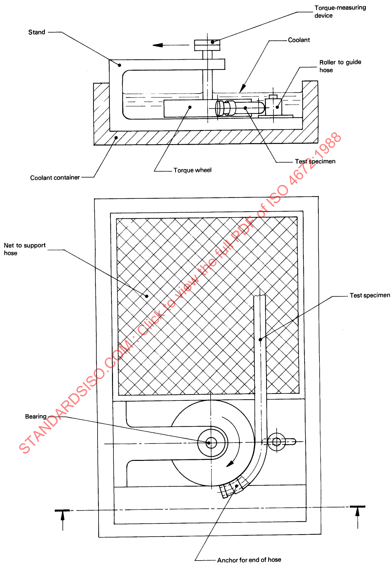
Figure 1 — Apparatus for method A
