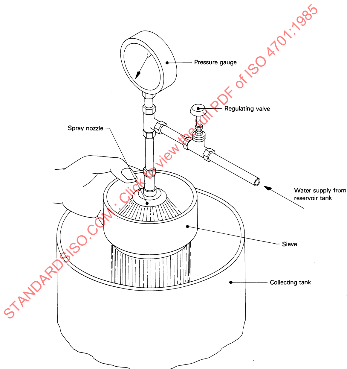
Figure 1 — A simple arrangement of wet sieving apparatus
