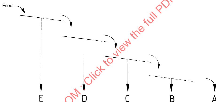
Figure 11 — Multi-deck, multi-drive, fine particles removed first
