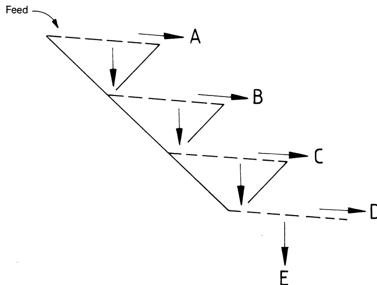
Figure 10 — Multi-deck, multi-drive, coarse particles removed first
