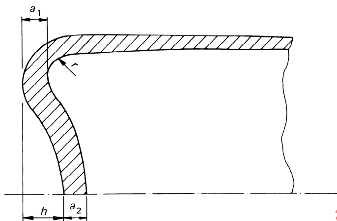
Figure 2 — Concave base end
