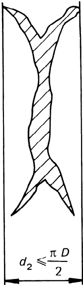
Figure 7 — Acceptable burst profile for quenched and tempered cylinders
