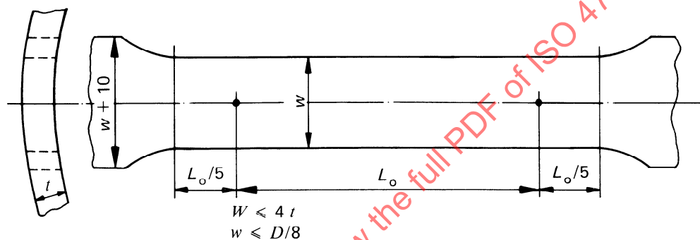
a) Test piece when t \geq 3 mm
