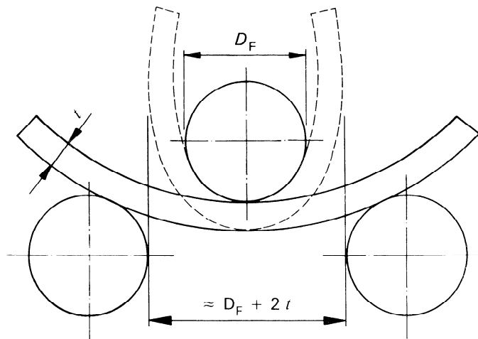
Figure 5 — Illustration of bend test
