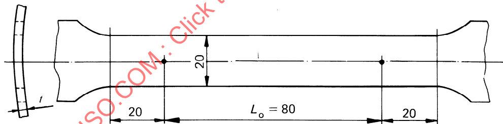
a) Test piece when t \geq 3 mm
