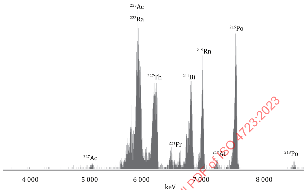
Figure A.3 — Spiked sample containing 15 mBq of ^{225}\text{Ac} tracer, 4 mBq of ^{227}\text{Ac} , counted 48 h, 40 days after separation
