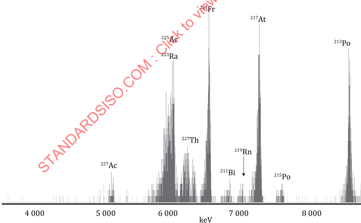
Figure A.2 — Spiked sample containing 15 mBq of ^{225}\text{Ac} tracer, 4 mBq of ^{227}\text{Ac} , counted 48 h shortly after separation
