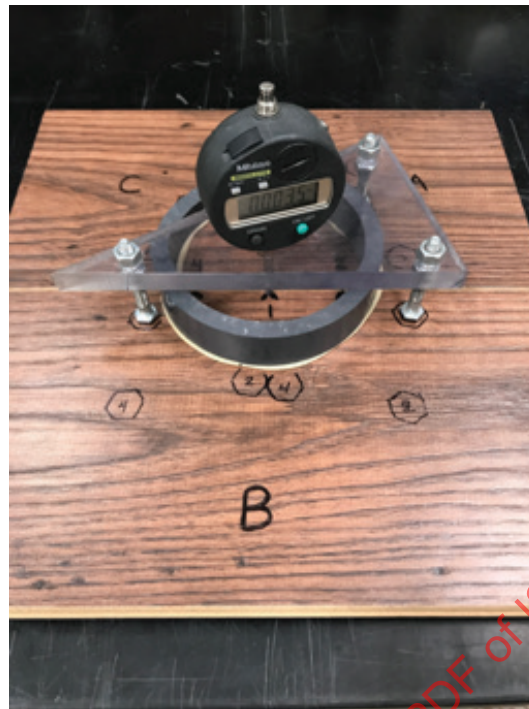
Figure 8 — Example of marked foot positions of measurement device
