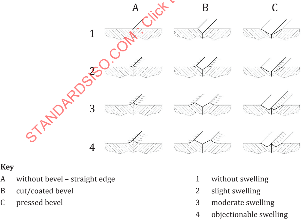
Figure 11 — Different swelling grades on different types of edges
