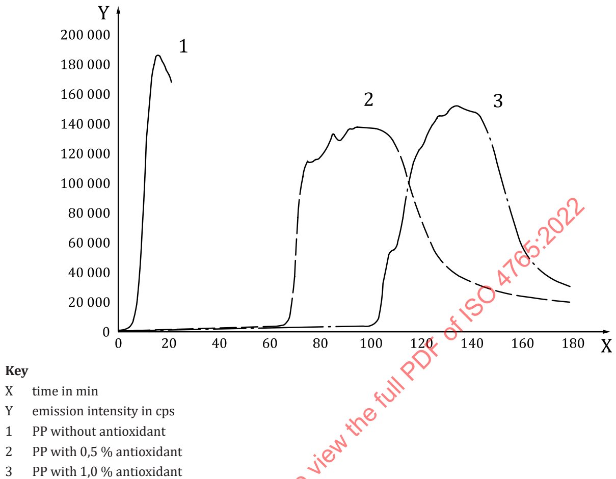
Figure D.1 — Example of change in oxidation induction time (OIT) of PP pellet with different concentration of antioxidants
