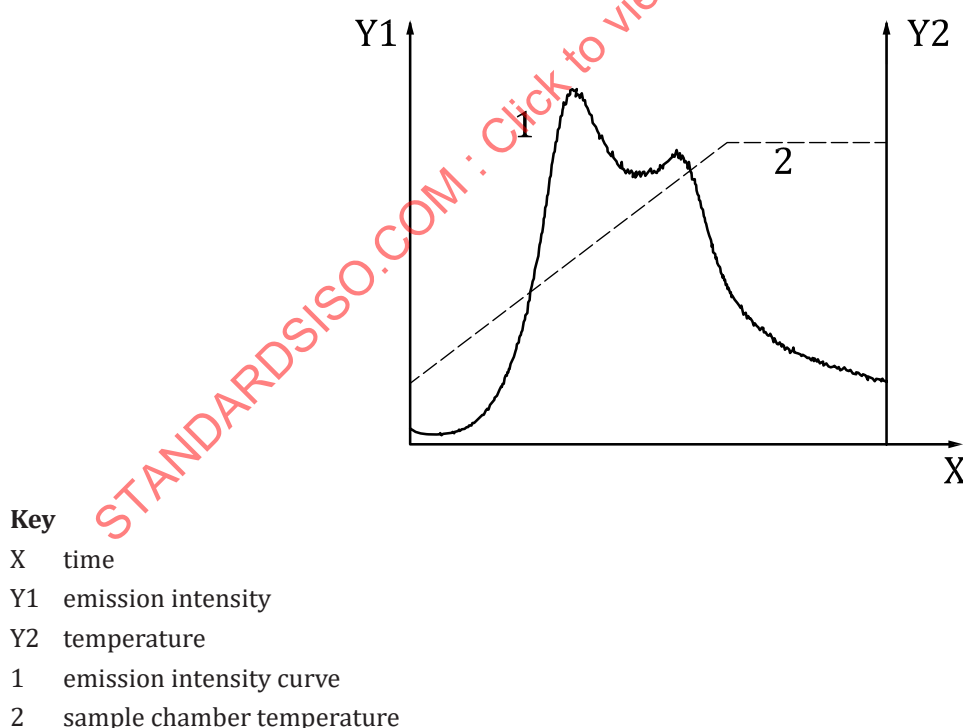
Figure 2 — Time course of emission intensity for non-isothermal measurement in inert gas atmosphere (example)
