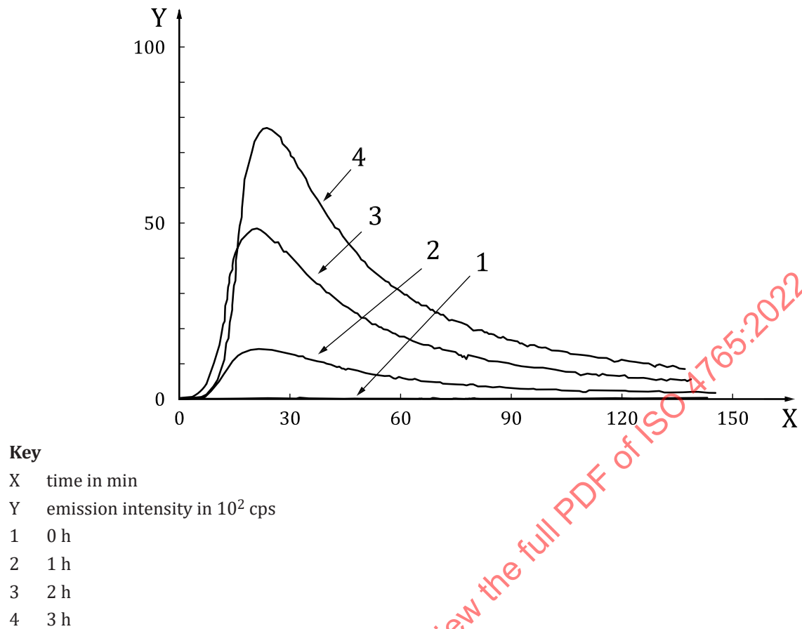
Figure C.1 — Example of UPE measurements of thermally oxidized polyethylene
