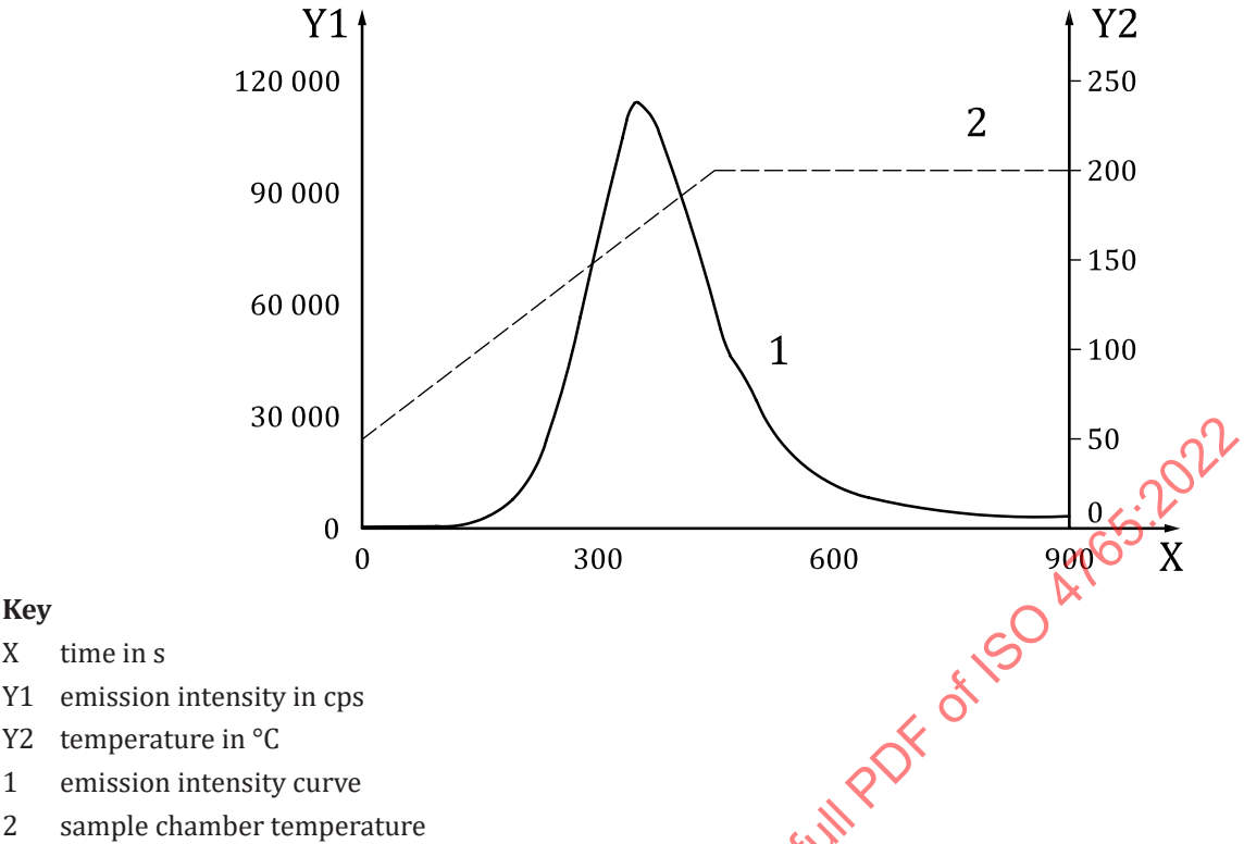
Figure B.1 — Example time course of UPE of thermally oxidized PP for non-isothermal measurement
