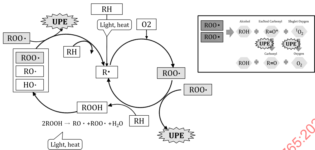
Figure A.2 — Autoxidation mechanism
