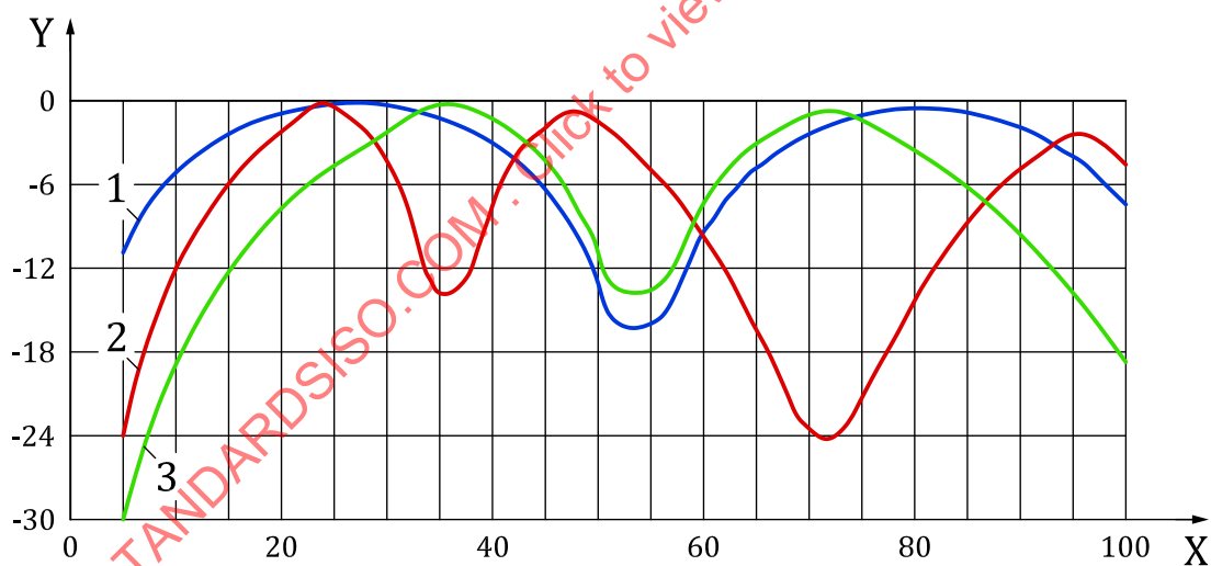
Figure A.4 — Effect of frequency and ring spacing on L(0,2) output
