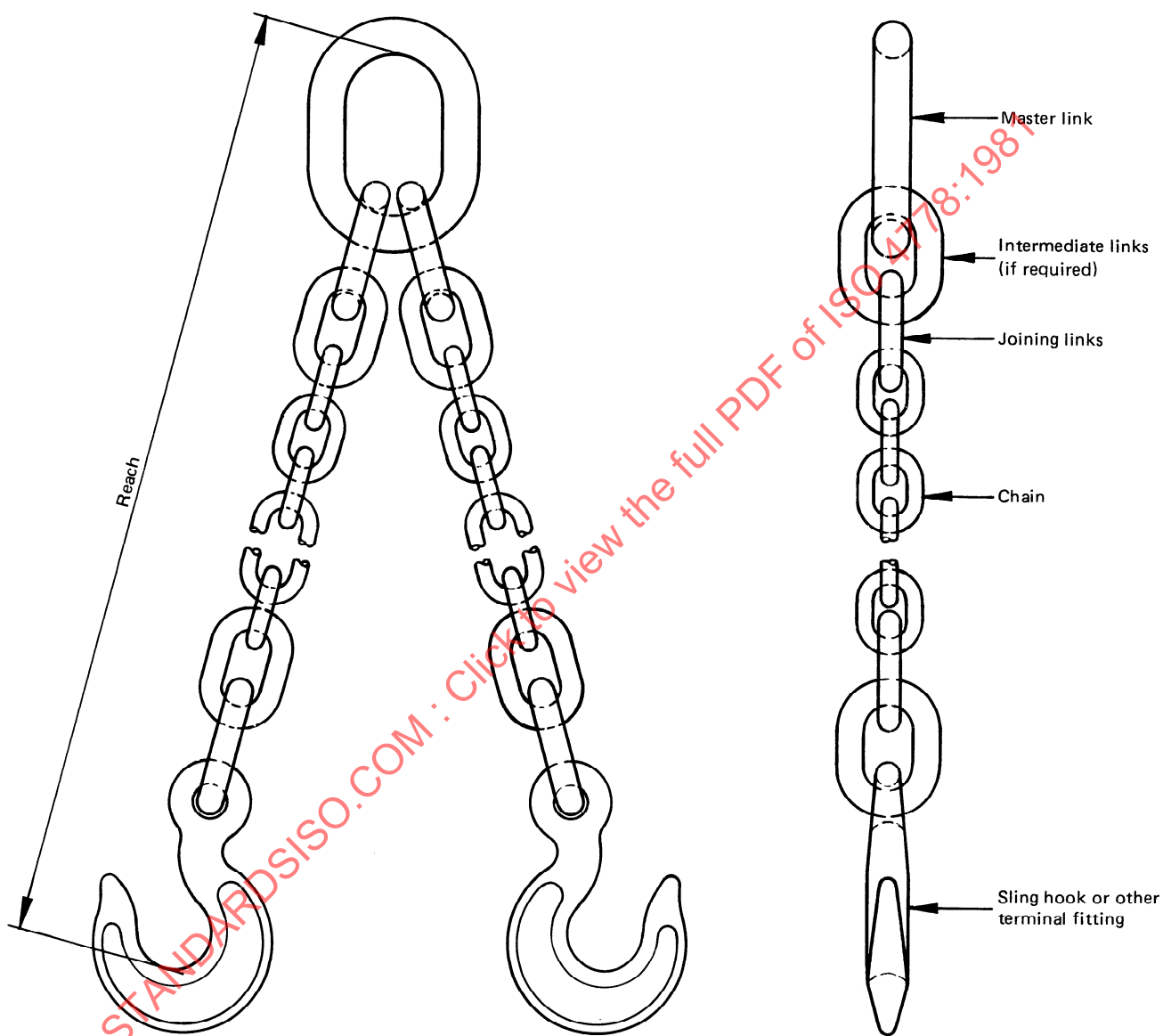
Figure 3 — Double branch sling
