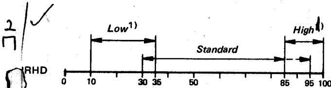
FIGURE 1 Range of applicability of hardness tests
