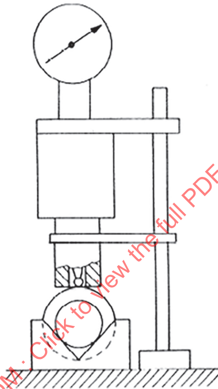
Figure 2 — Test jig for surfaces of small radius ( 4 \text{ mm} \leq R \leq 50 \text{ mm} )
