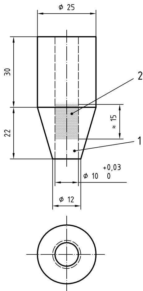
a) Dispensing tube a
