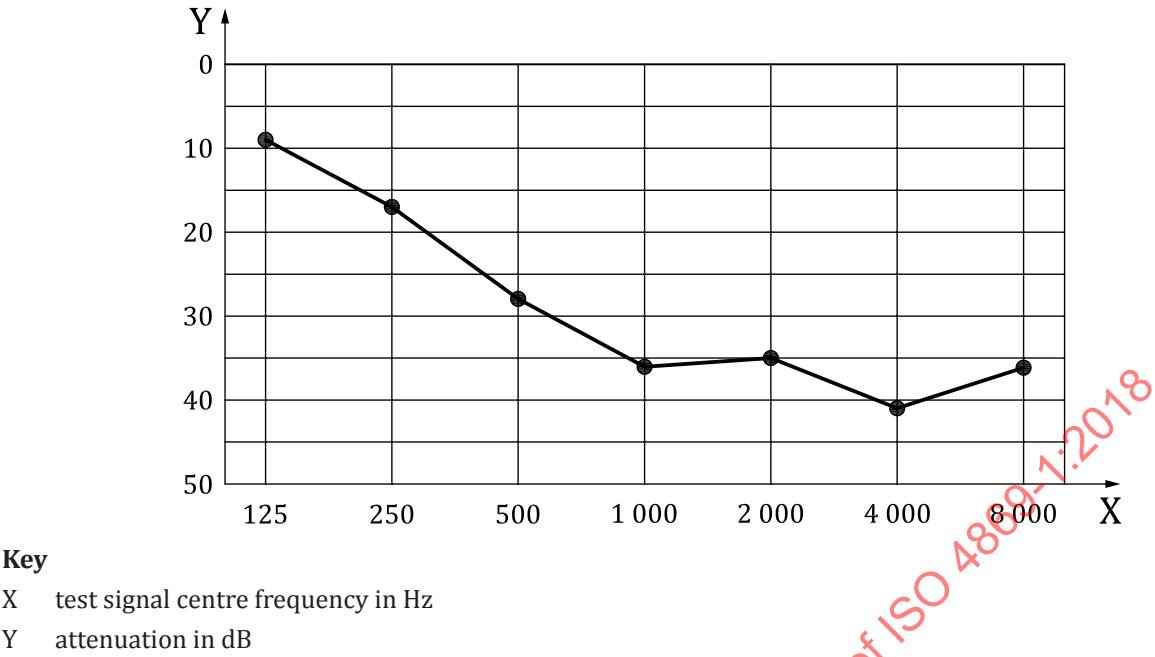
Figure 1 — Example of the mean attenuation of a hearing protector
