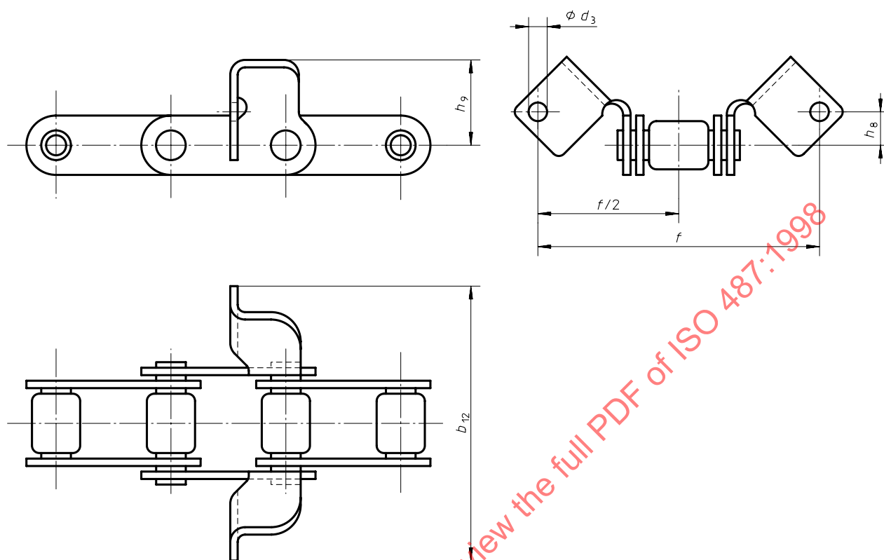
Figure 3 — F1 attachment plates
