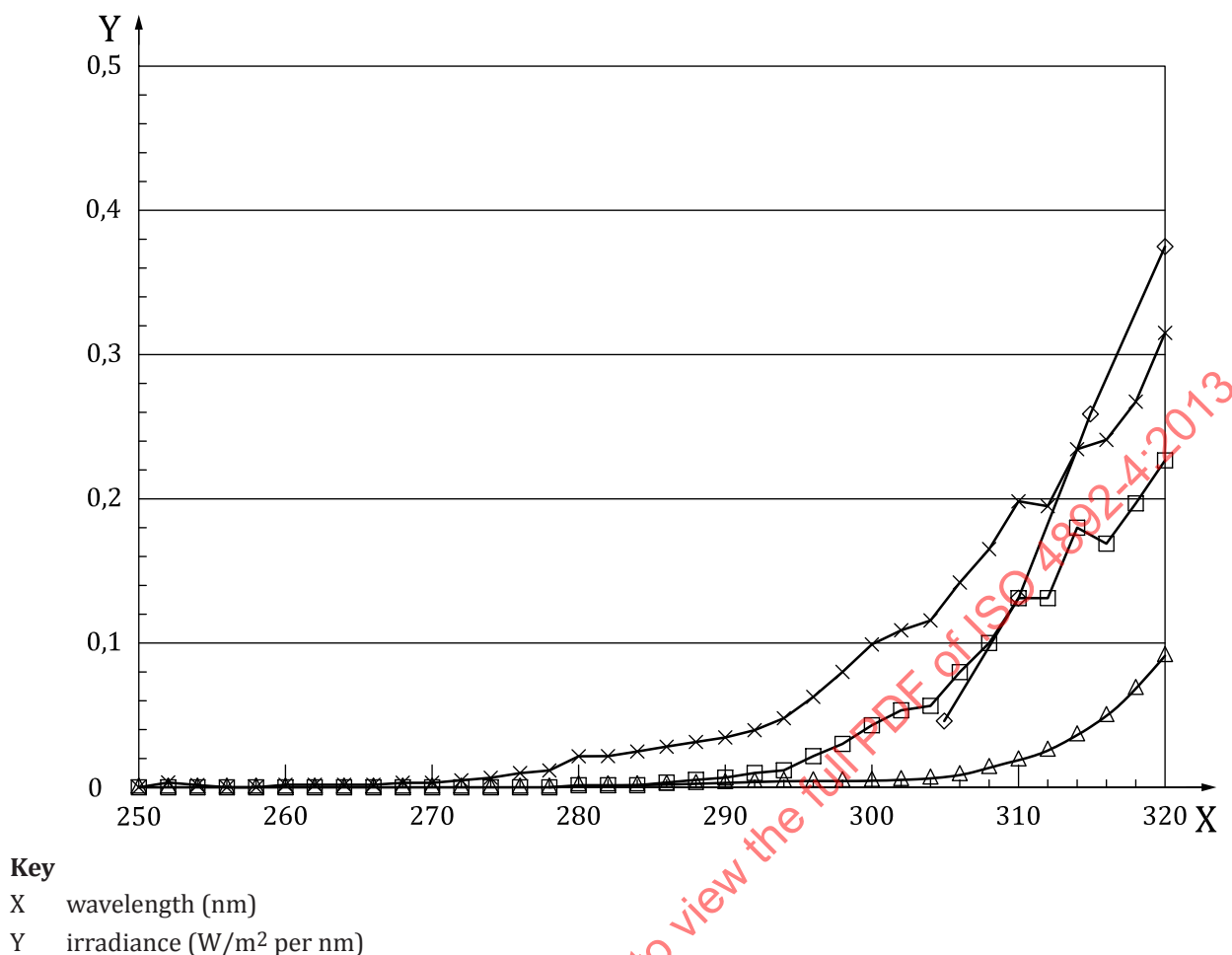
Figure 2 — Typical 250 nm to 320 nm spectral irradiance for open-flame carbon-arc lamps with type 1 filters (square symbols), type 2 filters (triangular symbols) and type 3 filters (crosses) compared to spectral irradiance of CIE 85:1989 Table 4 daylight (diamond-shaped symbols)
