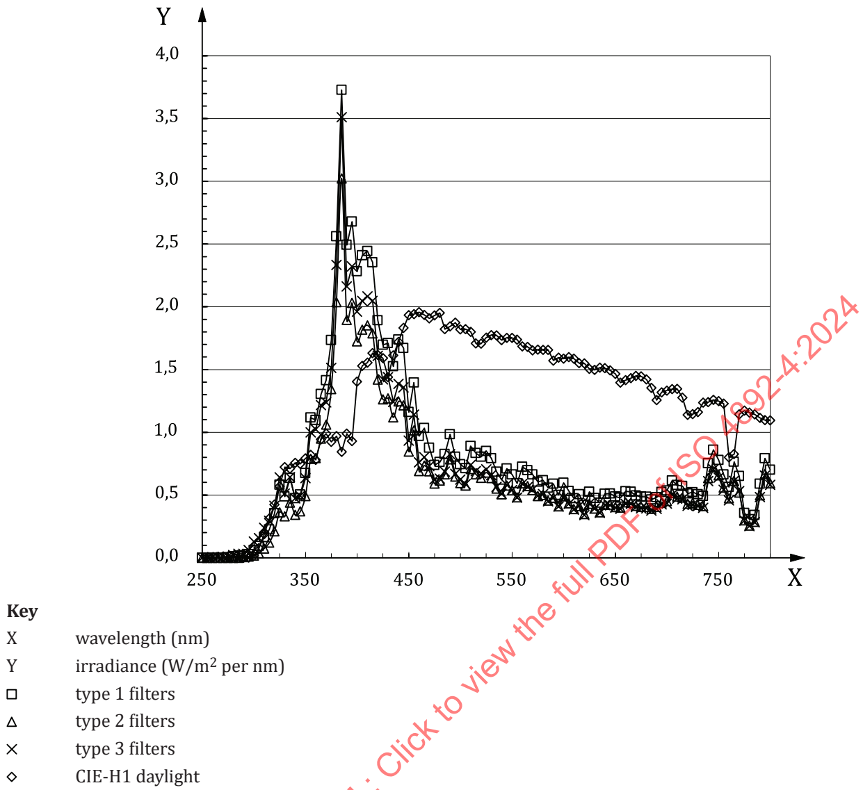
Figure 1 — Typical spectral irradiance for open-flame carbon-arc lamps with type 1 filters, type 2 filters and type 3 filters compared to spectral irradiance of CIE 241, CIE-H1 daylight
