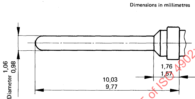
Figure 6 — Male contact
