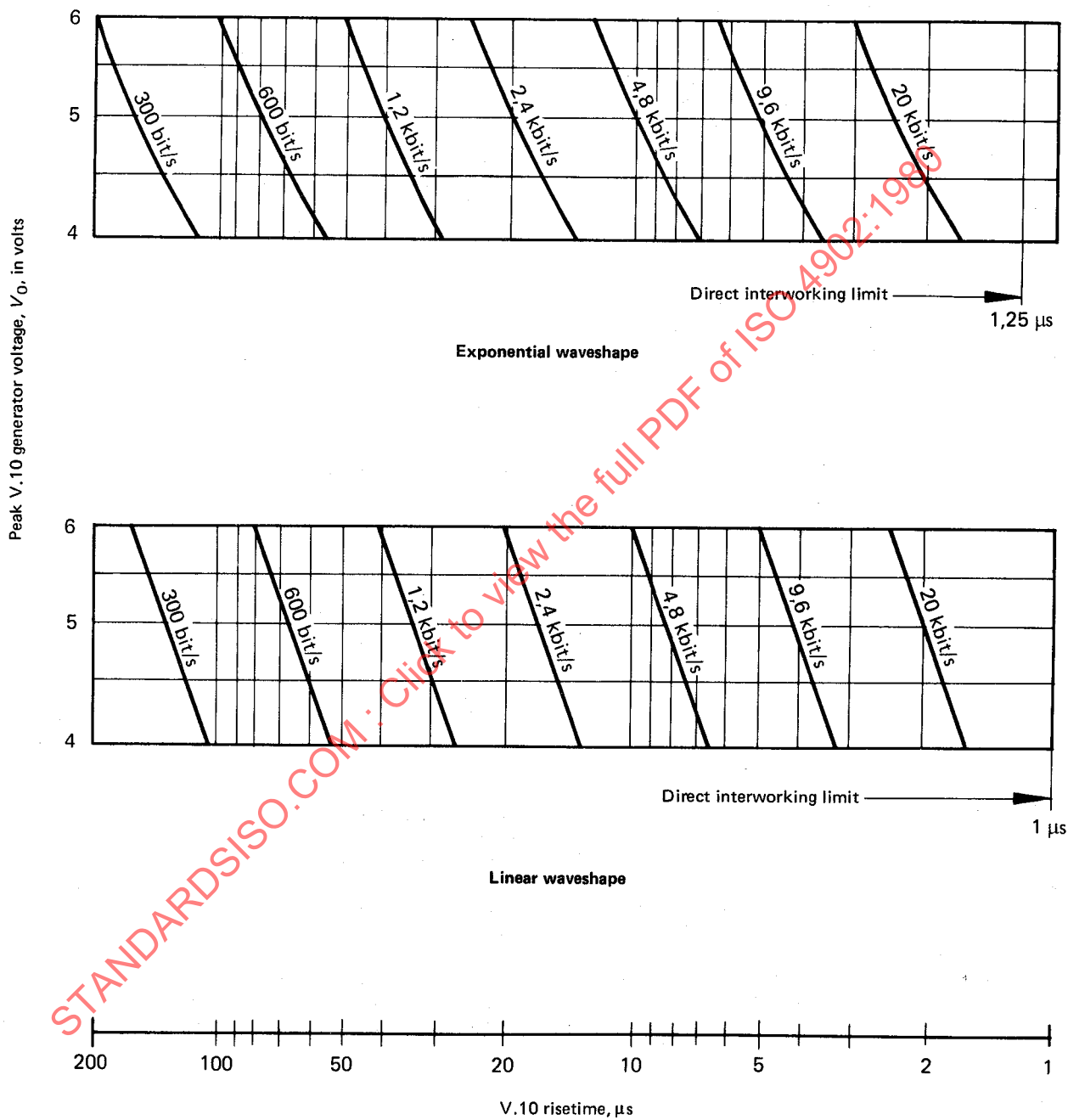
Figure 10 — Risetime relationship to V.10/V.28 interworking
