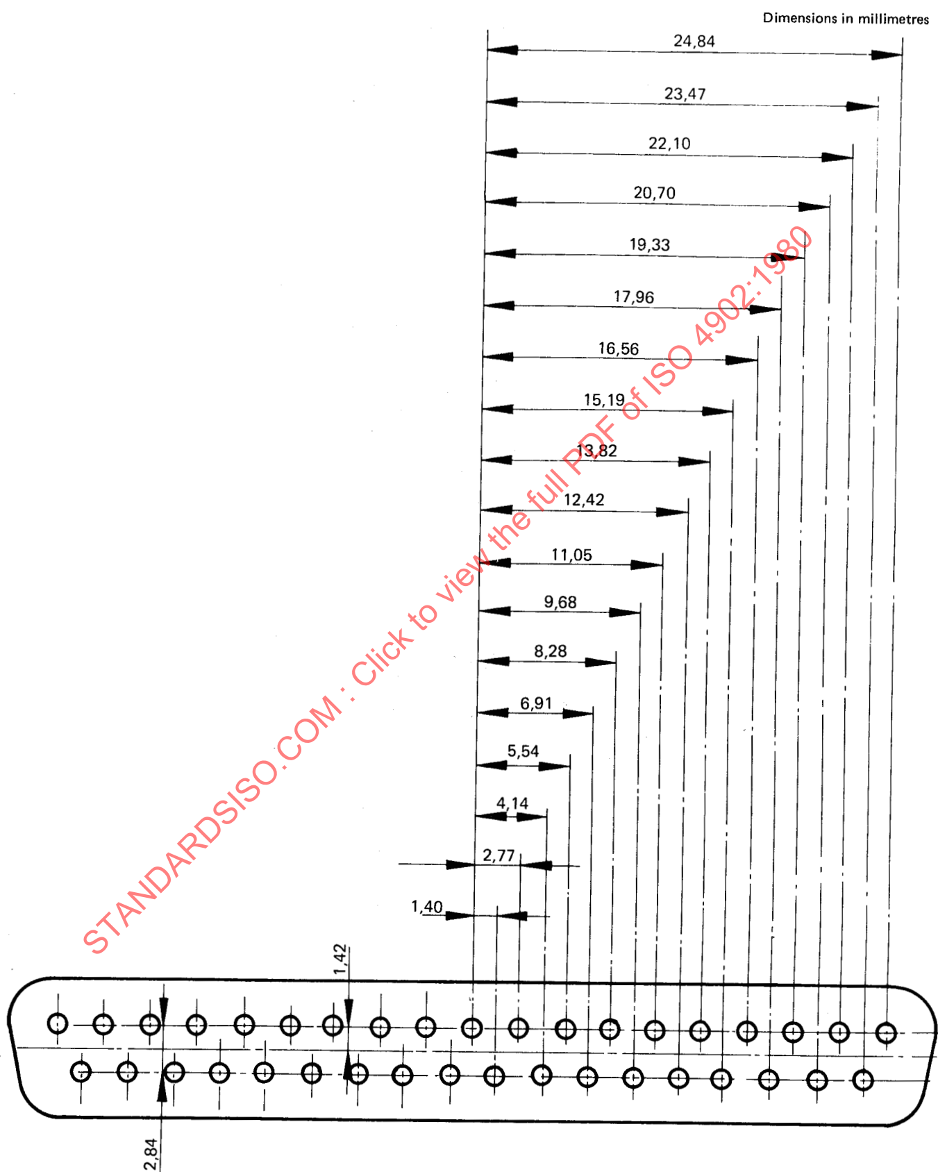
Figure 5a) — 37-pin insert arrangement
