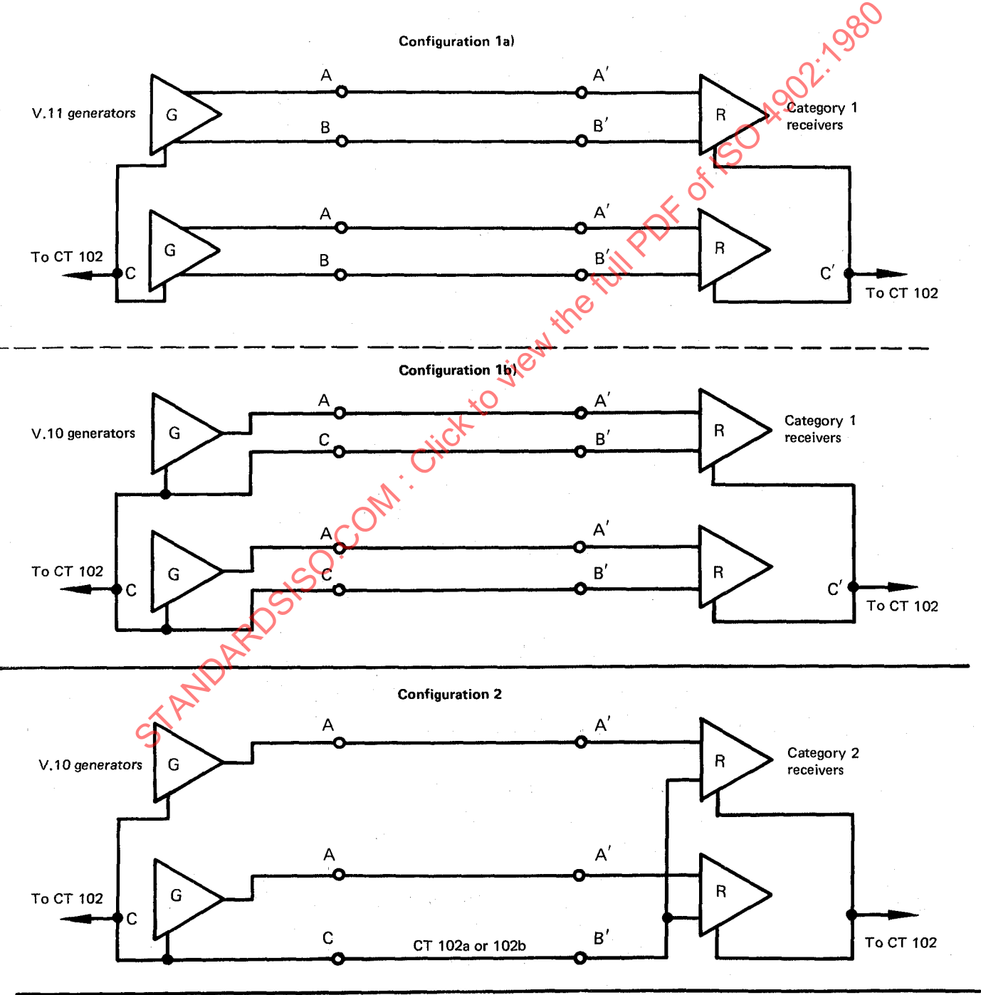
Figure 8 — Generator/receiver interconnecting configurations
