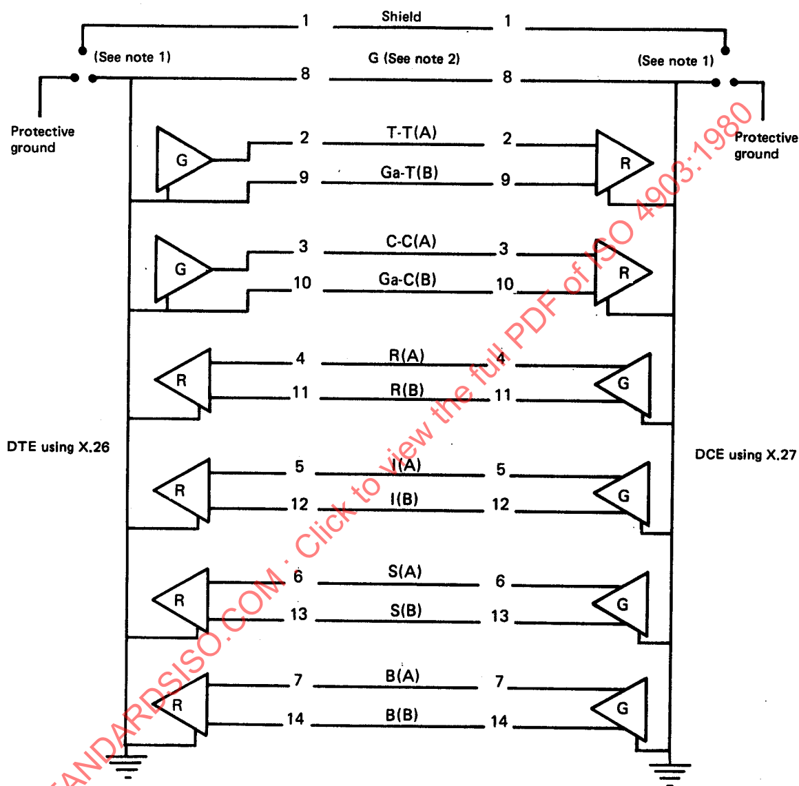
Figure 10 — X.21 interconnection configuration for X.26 DTE/X.27 DCE
