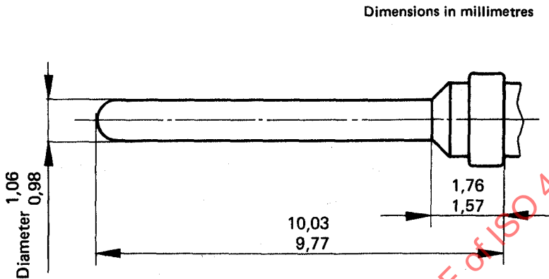
Figure 6 — Male contact
