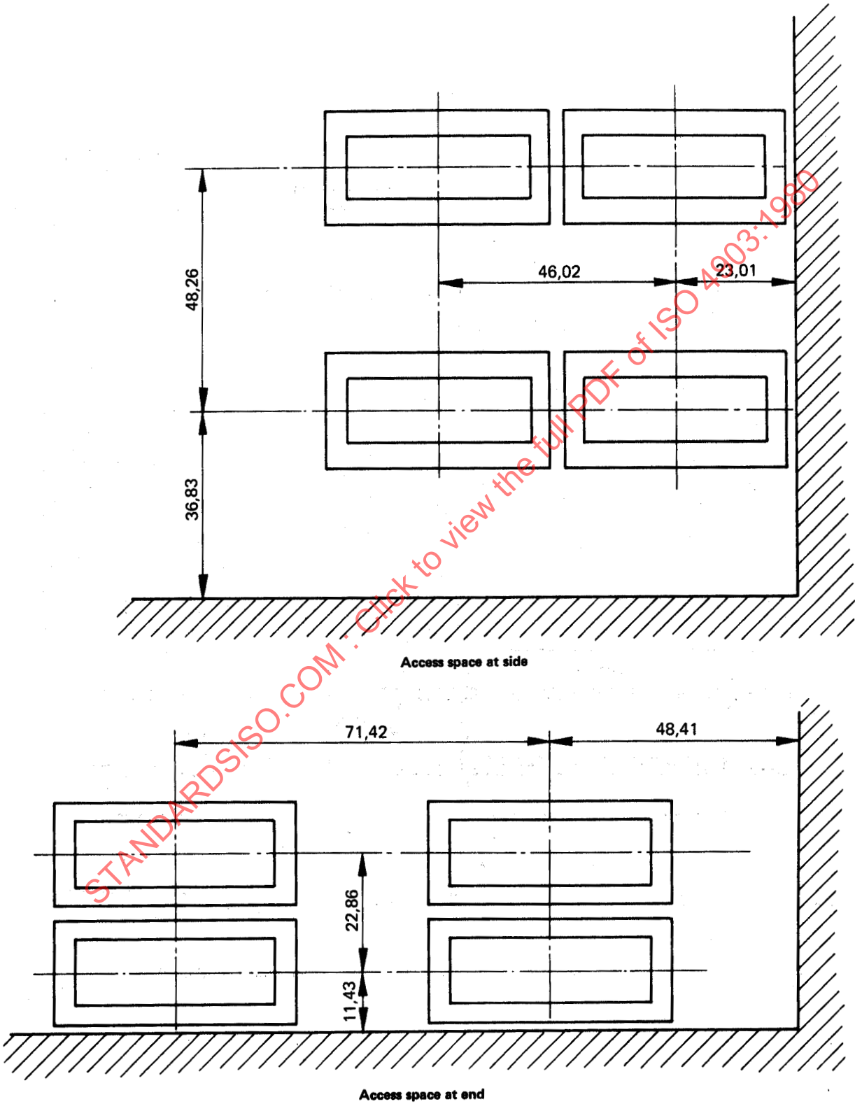
Figure 4 — Minimum spacing for DCE connector mounting
