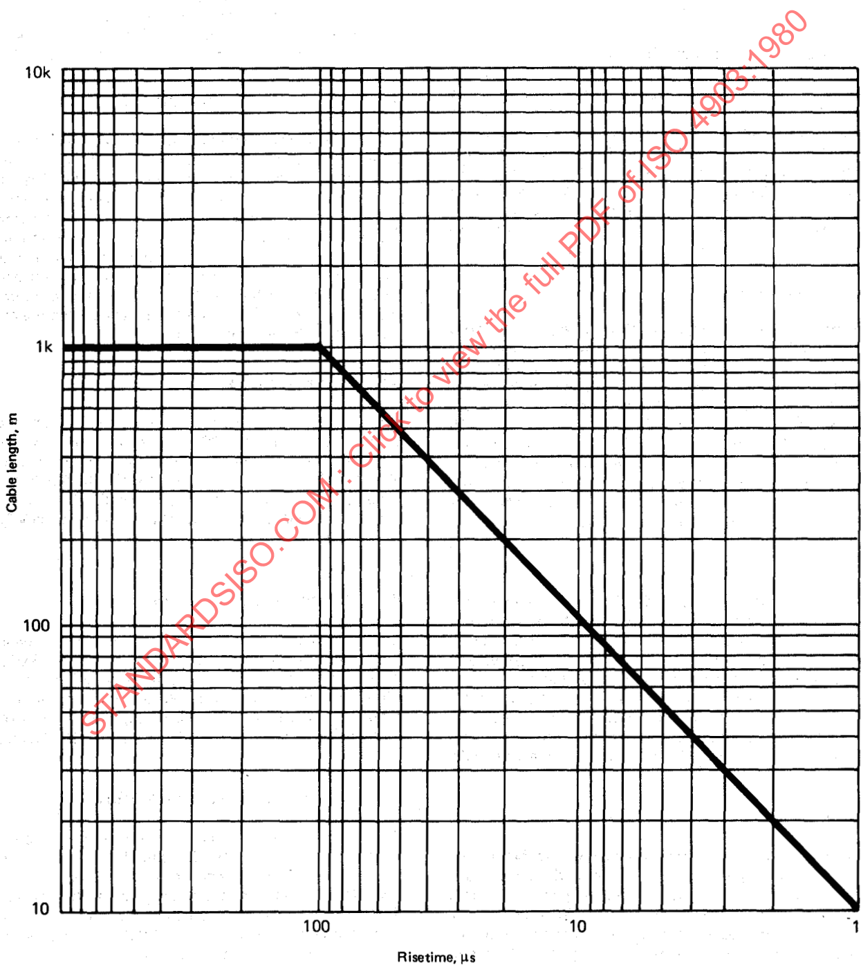
Figure 12 — Cable length against risetime
