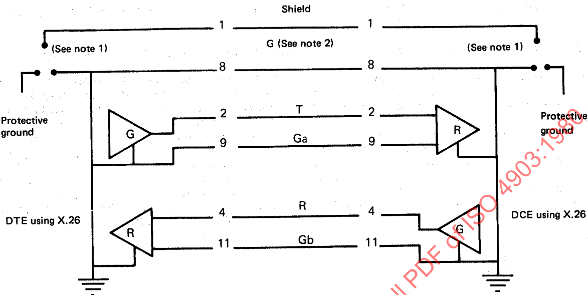
Figure 8 — X.20 interconnection configuration for X.26 DTE/X.26 DCE
