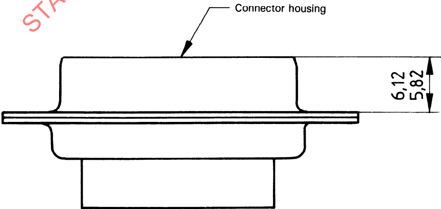
Figure 1 — DTE connector
