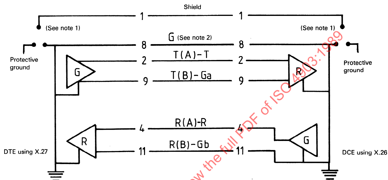
Figure B.2 — X.20 interconnection configuration for X.27 DTE/X.26 DCE
