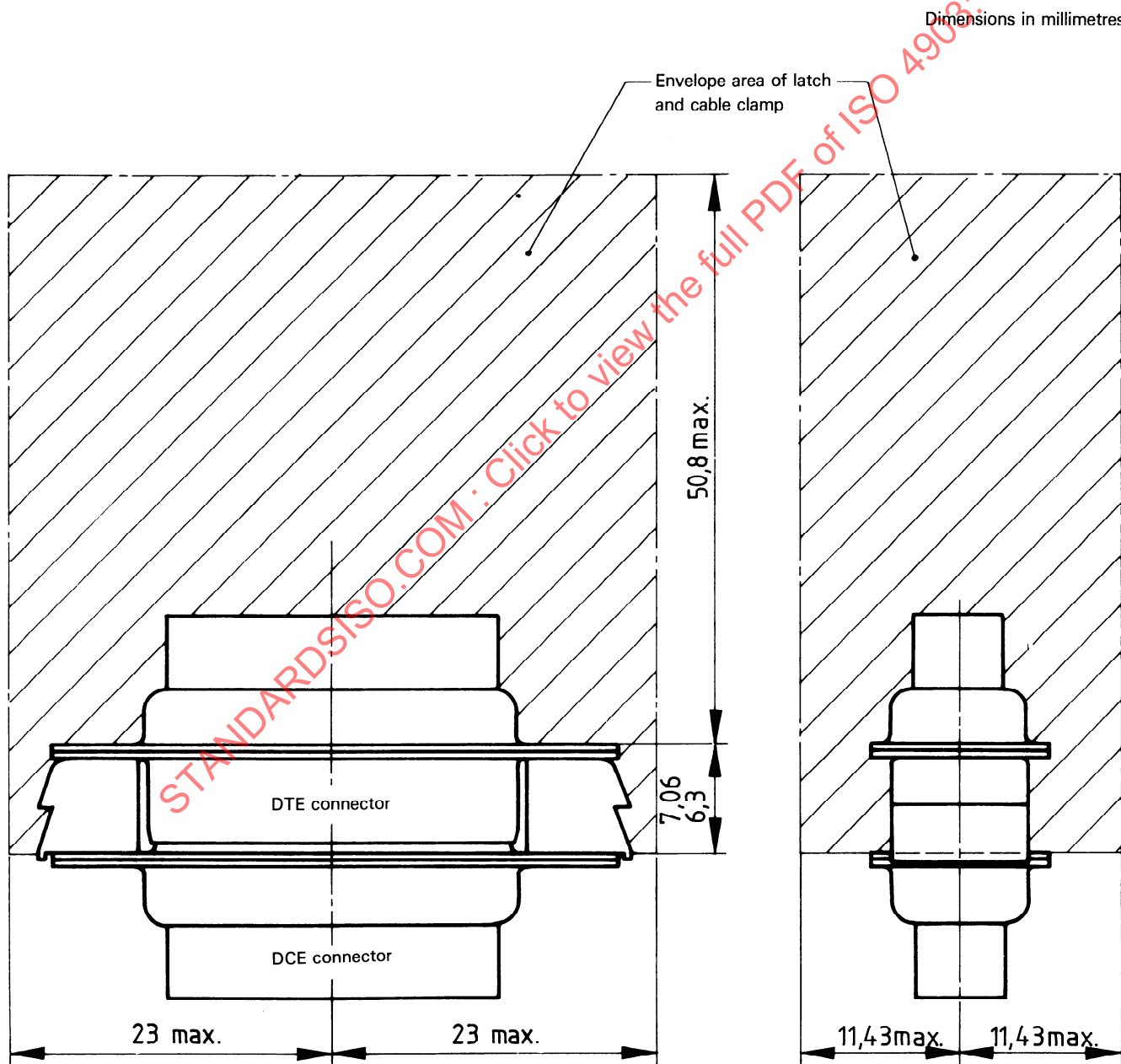
Figure A.1 — Maximum DTE connector outline
