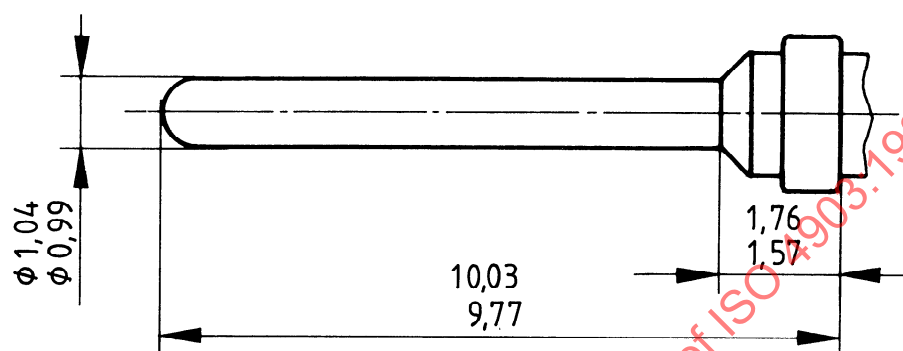
Figure 4 — Male contact
