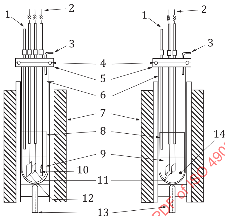
a) Three-electrode system for polarization and EIS measurements
