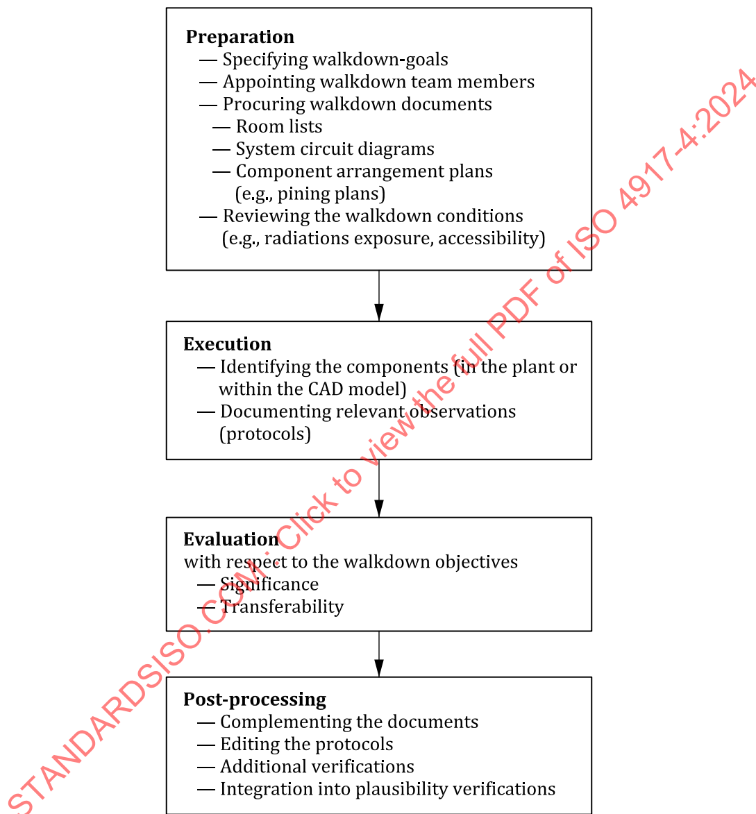
Figure 4 — Schematic sequence of walkdown inspections
