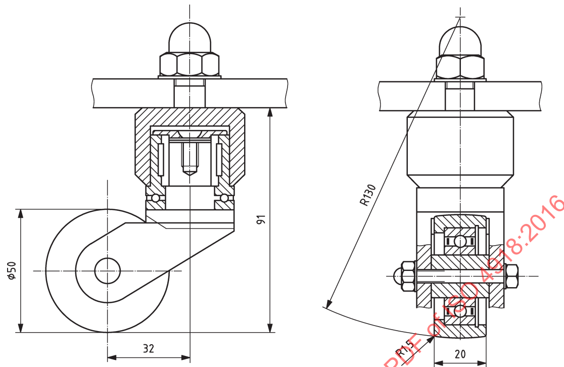
Figure 3 — Single-wheel swivel castors (nominal dimensions in mm)
