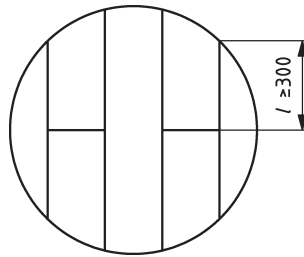
Figure 5 — Example of an assembled test area of laminate floor coverings
