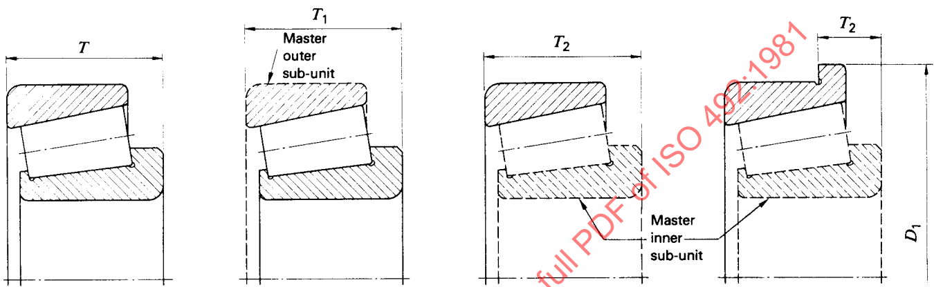
Figure 2 — Additional symbols for tapered roller bearings
