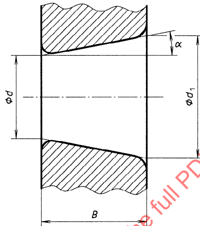
Figure 3 — Nominal tapered bore
