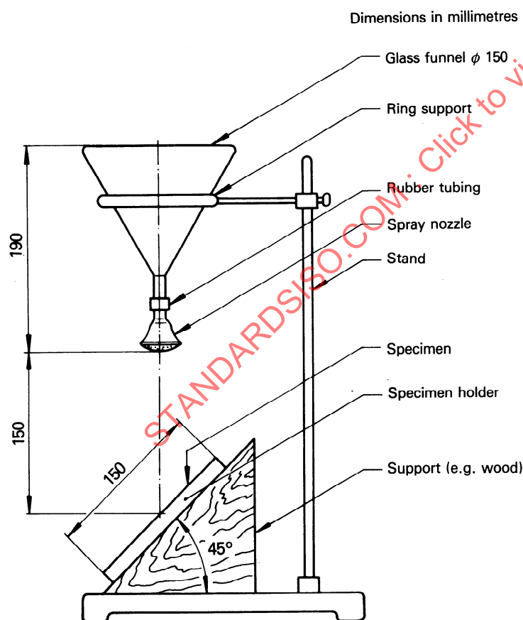
Figure 1 — Apparatus for spray test
