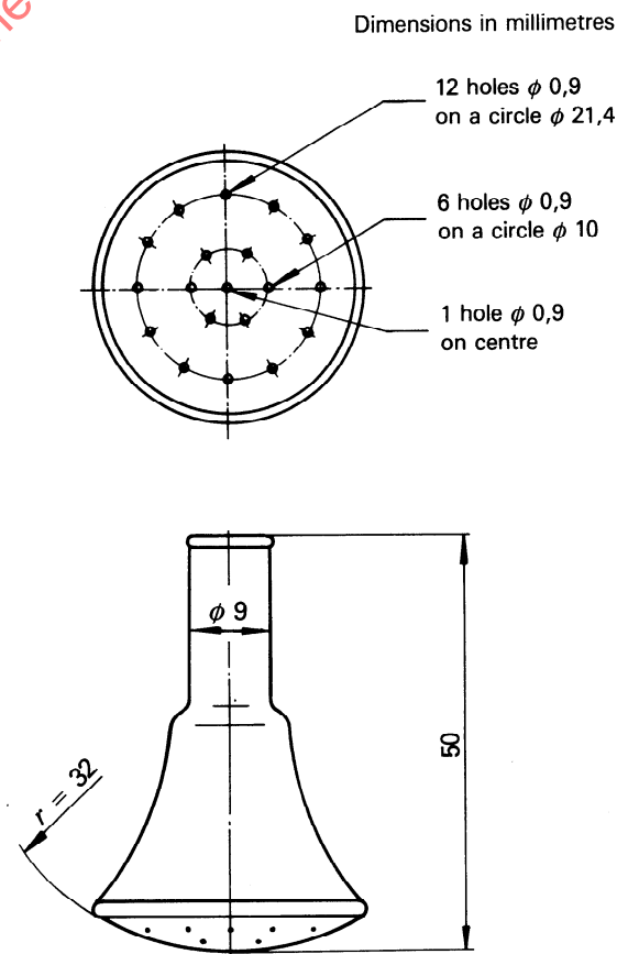
Figure 2 — Spray nozzle
