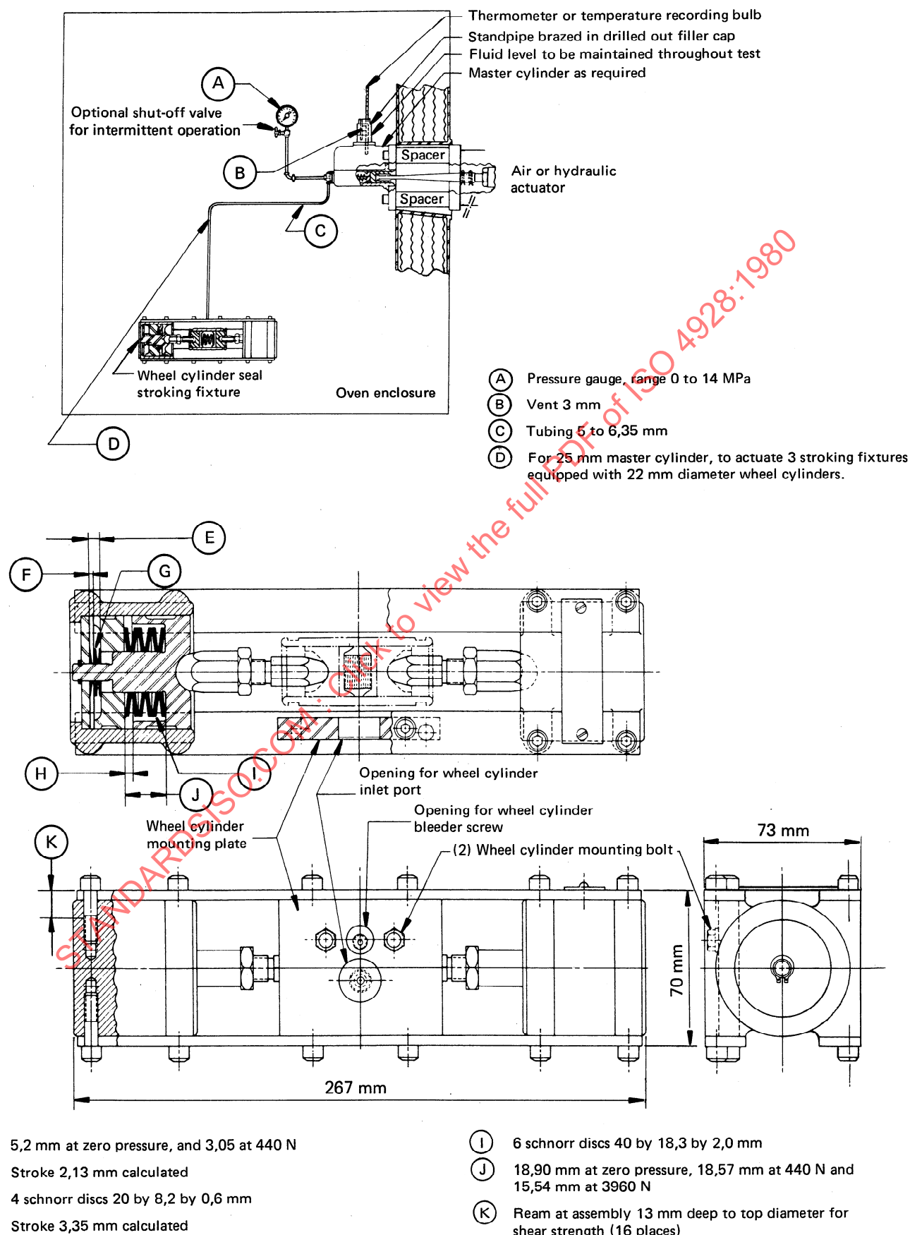
Figure 1 — Recommended wheel and master cylinder stroking test apparatus
