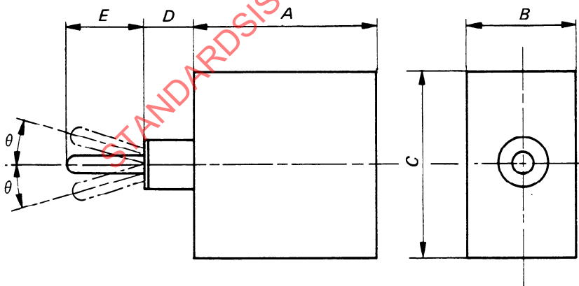
FIGURE 1 – Dimensions for single-hole mounting switch
