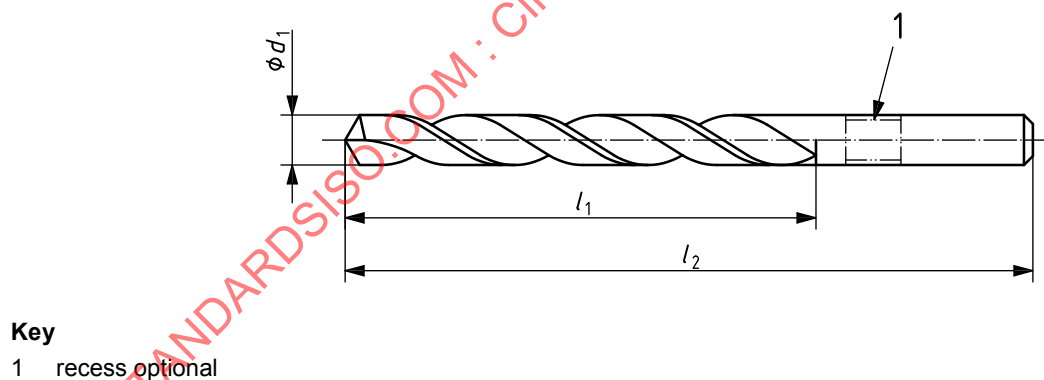
Figure 1 — Dimensions of cylindrical shank twist drill
