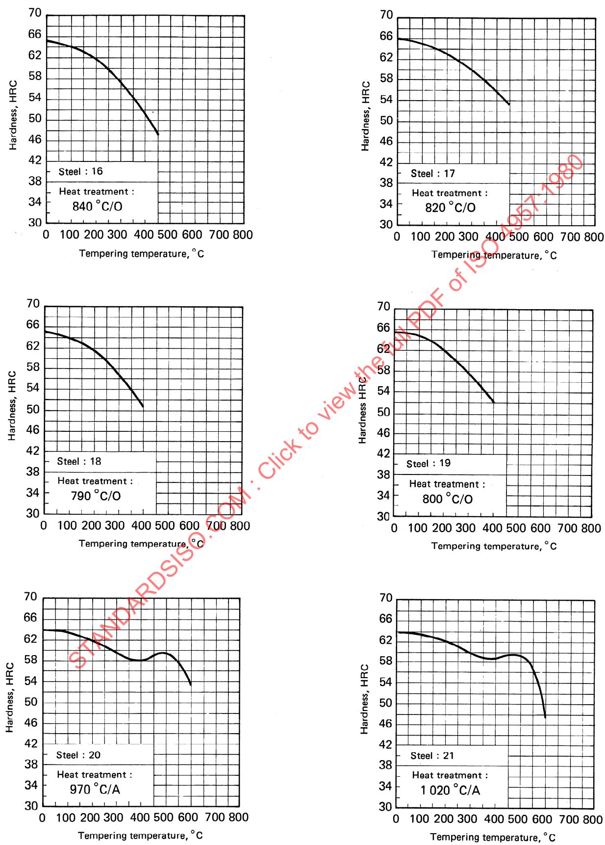
Figure 2b — Hardness-tempering temperature-curves for alloyed cold-work tool steels (see table 4 and 3.6.3)
