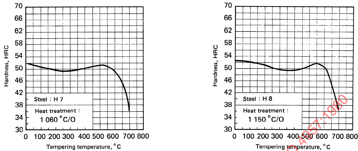
Figure 3b — Hardness-tempering temperature-curves for hot-work tool steels (see table 6 and 3.6.3)
