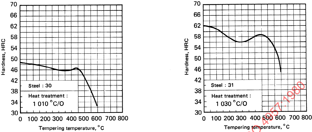
Figure 2d — Hardness-tempering temperature-curves for alloyed cold-work steels (see table 4 and 3.6.3)
