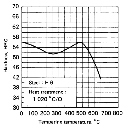
Figure 3a — Hardness-tempering temperature-curves for hot-work tool steels (see table 6 and 3.6.3)
