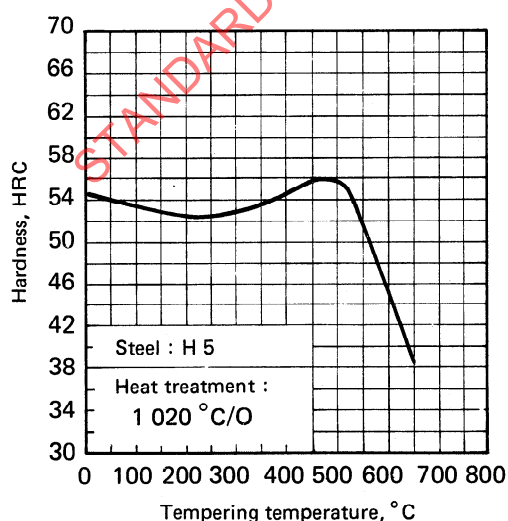
Figure 3a — Hardness-tempering temperature-curves for hot-work tool steels (see table 6 and 3.6.3)
