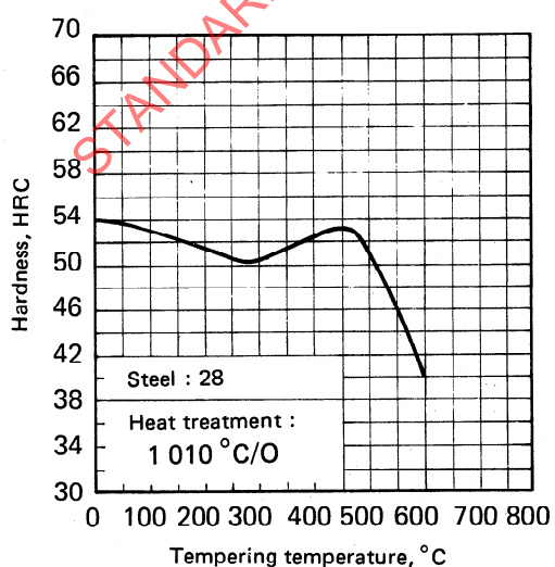
Figure 2c — Hardness-tempering temperature-curves for alloyed cold-work tool steels (see table 4 and 3.6.3)
